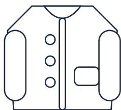
Coat on
