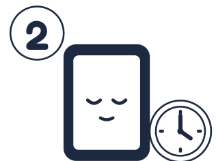
Screens later
