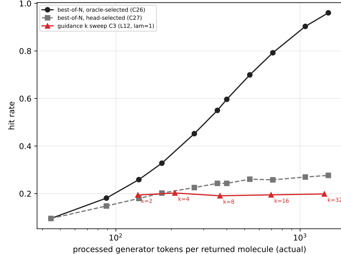
qed
