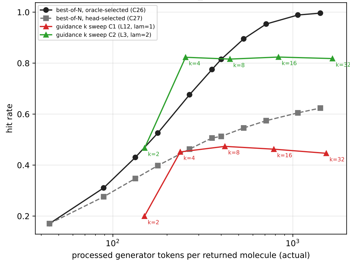
aromatic_rings
