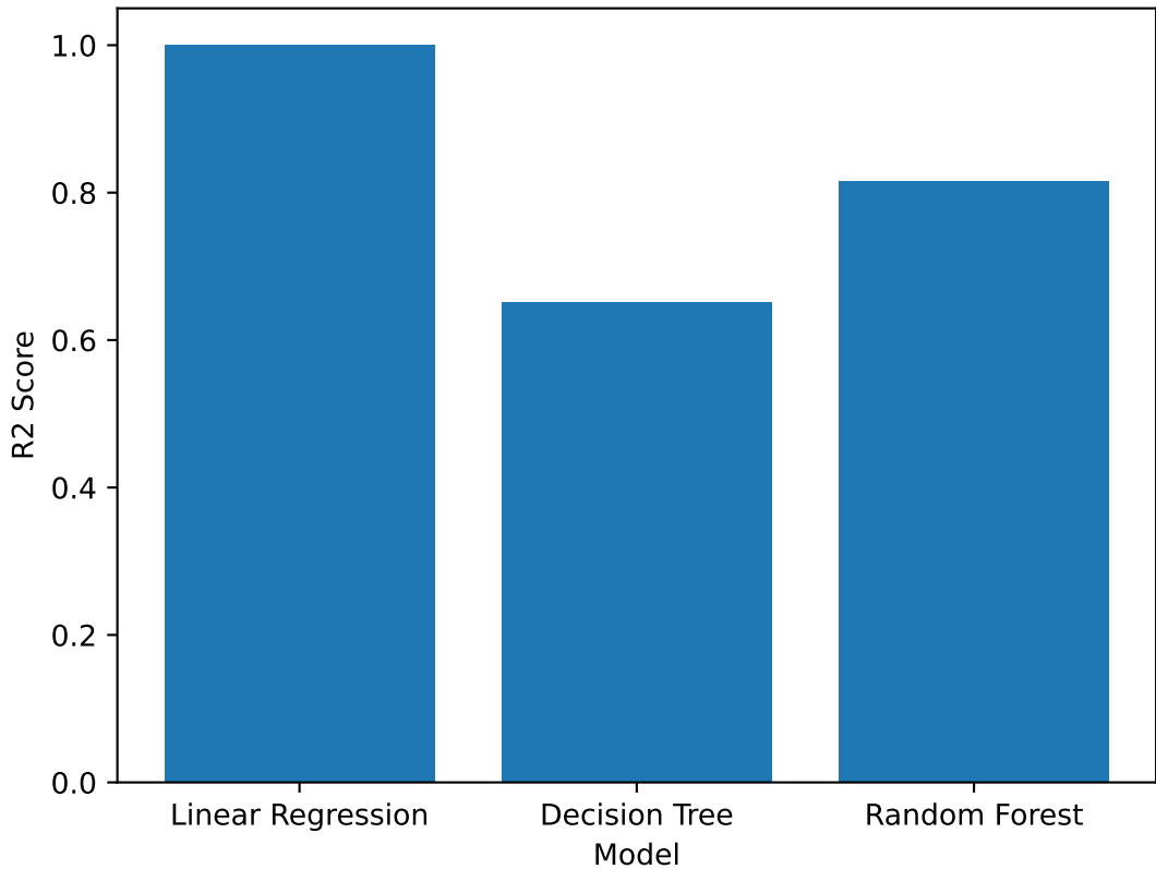
Model Comparison (R2 Score)
