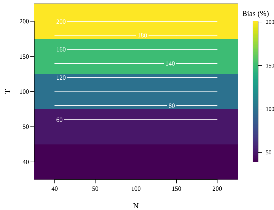
(c) Bias Surface: CS Estimator
