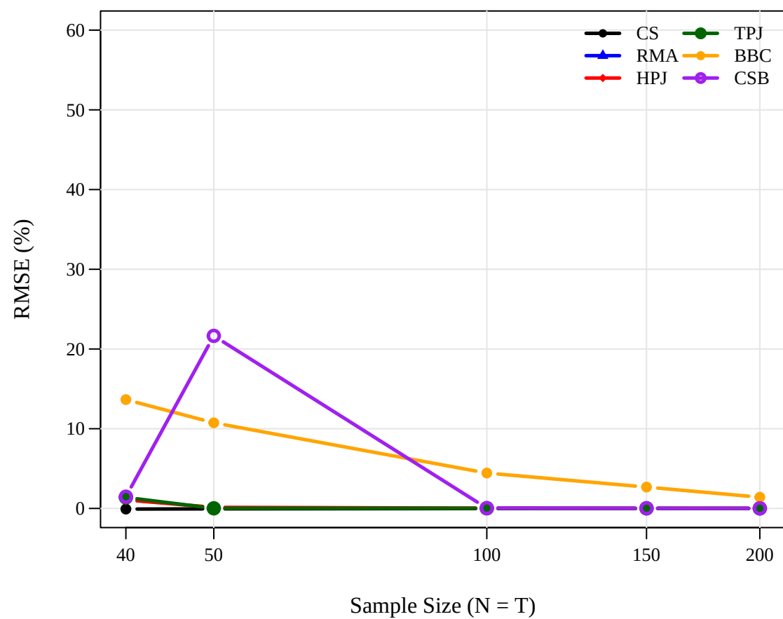
(b) RMSE Convergence Across Methods
