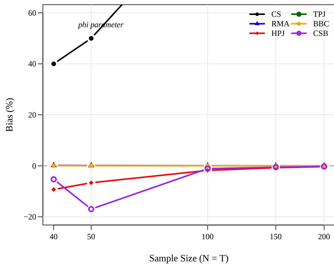
(a) Bias Convergence Across Methods
