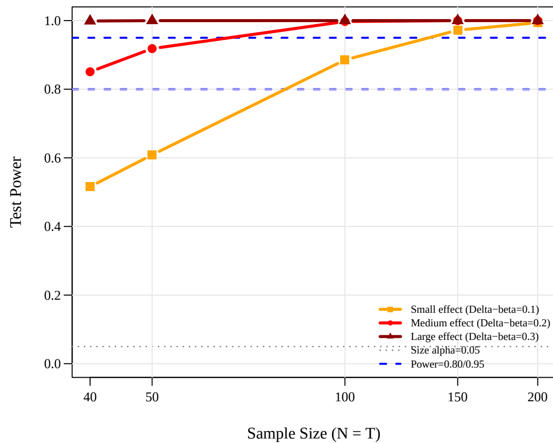
(c) Asymmetry Test Power (H0: \theta_+ = \theta_- )
