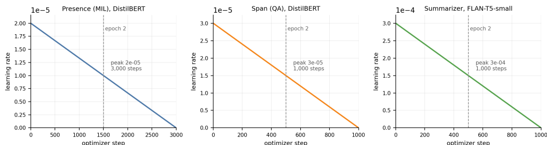
Figure 4.9: Learning-rate schedules
