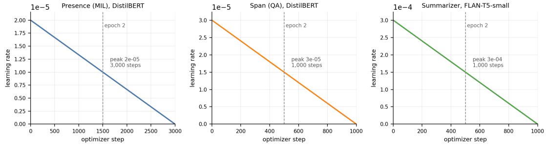
Figure 4.9: Learning-rate schedules
