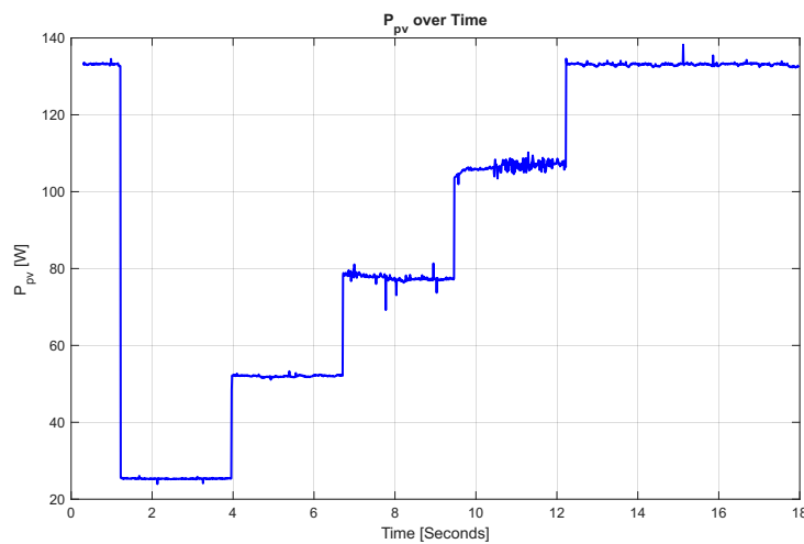
Figure 6.12: PV Power over time with steps of 200 W/m 2 , from 200 to 1000 W/m 2 .
