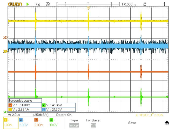
Figure 6.4: Measured waveforms before adding the additional ceramic capacitors.
