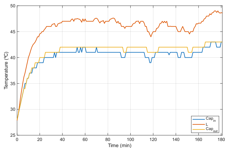
Figure 6.9: Temperature evolution during 3 hours. Preciso do DBC para adicionar o T_{fets} e o T_{amb}
