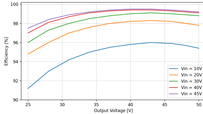
Figure 6.11: Converter efficiency over output voltage for different input voltages. Just a place holder image. No real data!!
