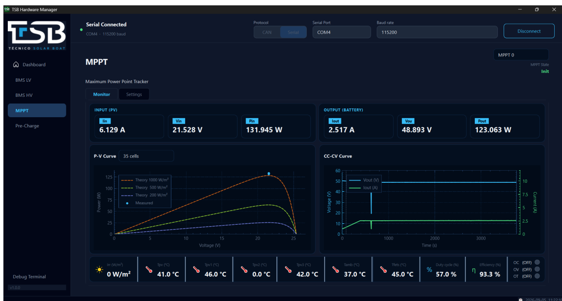
Figure 4.9: MPPT tab.
