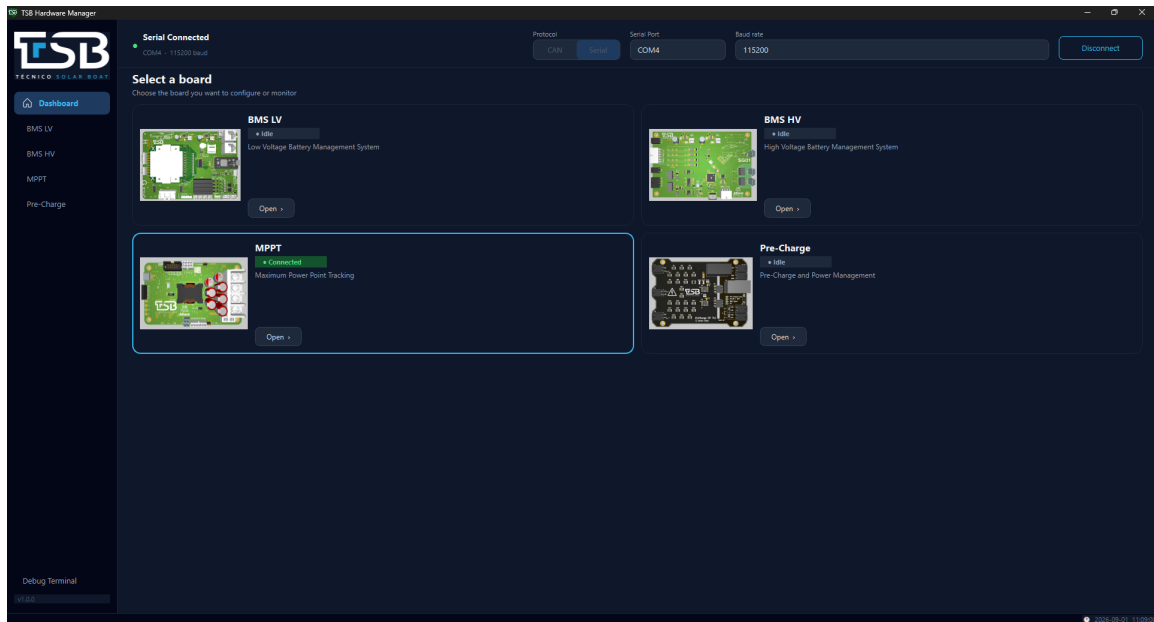
Figure 4.8: Dashboard page.
