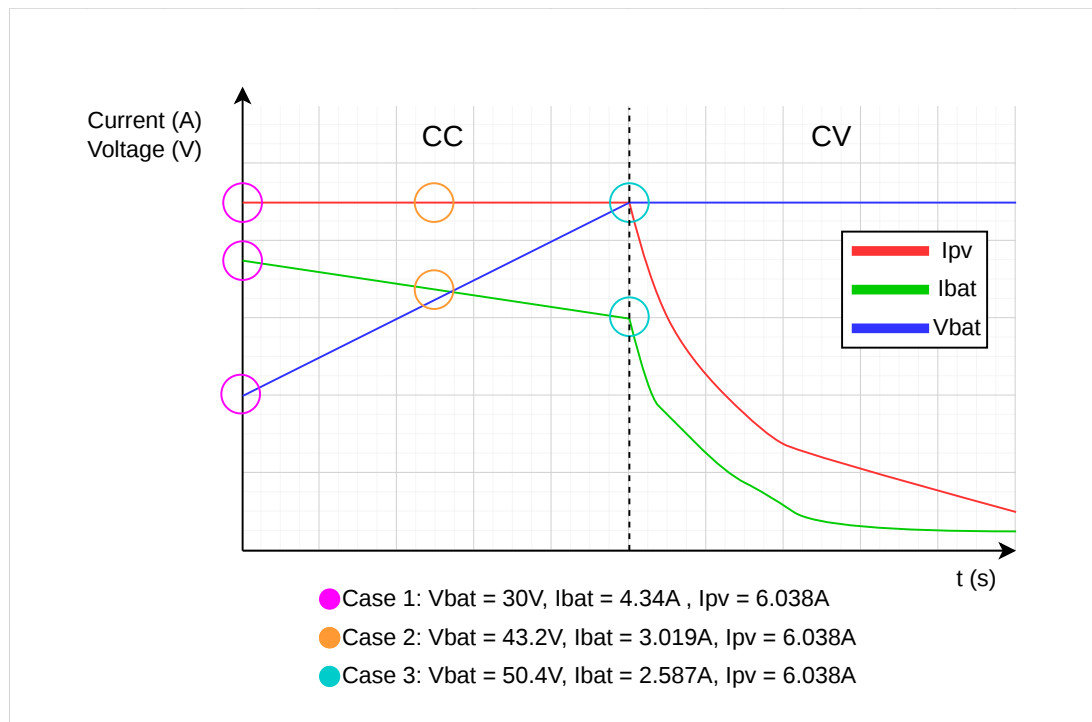
Figure 5.3: CC-CV charge characteristics and case selection.
