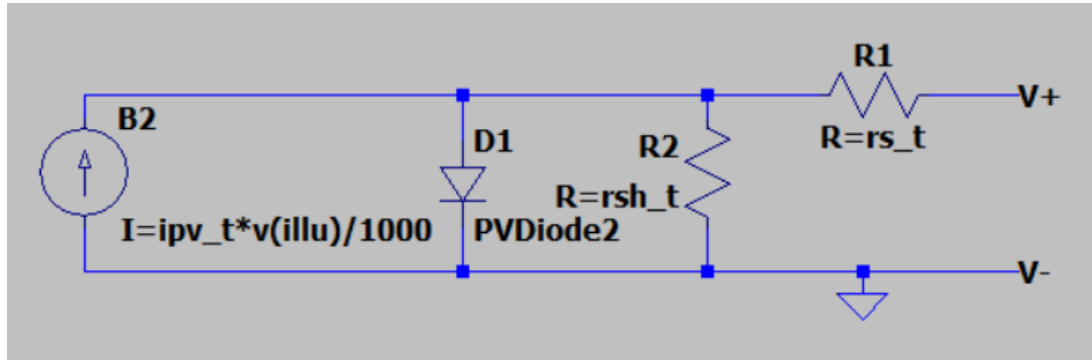
Figure 5.2: Solar panel model diagram (1M5P configuration).
