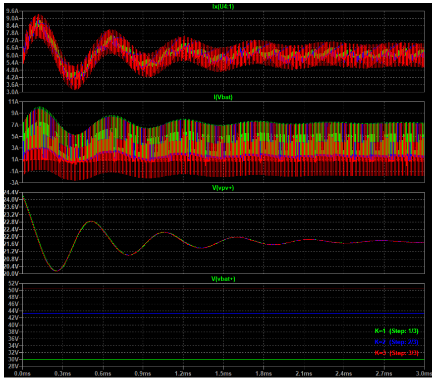
Figure 5.6: 3 stages of charge waveforms.
