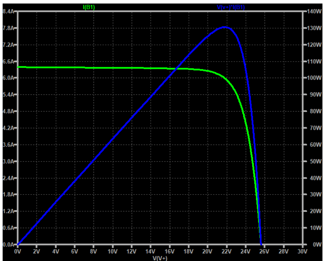
Figure 5.1: I-V and P-V characteristics of a solar panel model with 35 cells in series.
