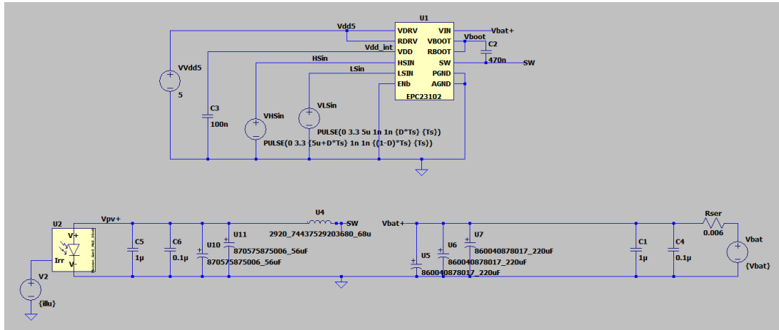
Figure 5.4: Simulation circuit diagram.
