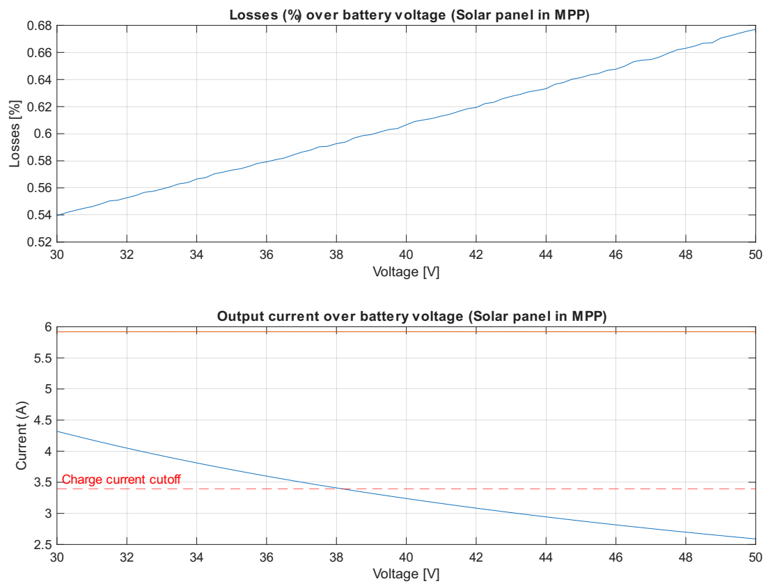
Figure 5.5: Battery voltage sweep simulation results.
