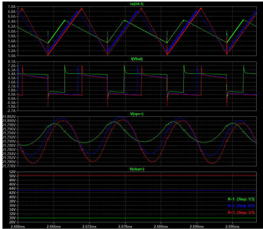
Figure 5.7: 3 stages of charge waveforms in zoomed view.
