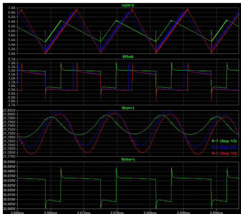
Figure 4.10: 3 stages of charge waveforms in enhanced zoomed view.
