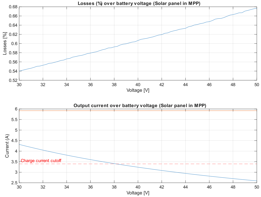
Figure 4.7: Battery voltage sweep simulation results.
