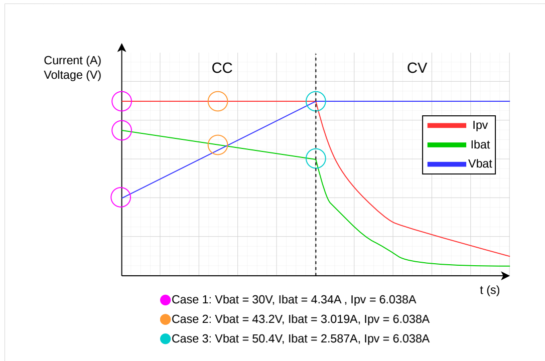
Figure 4.5: CC-CV charge characteristics and case selection with V_{mpp} = 21.595 V .
