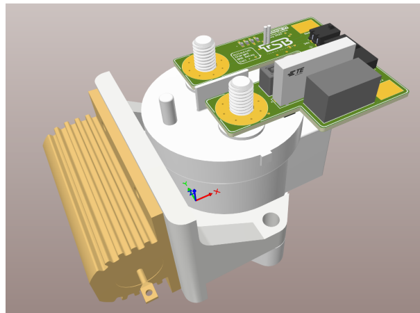
Figure 4.14: Precharge 3D design.
