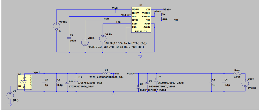
Figure 4.6: Simulation circuit diagram.
