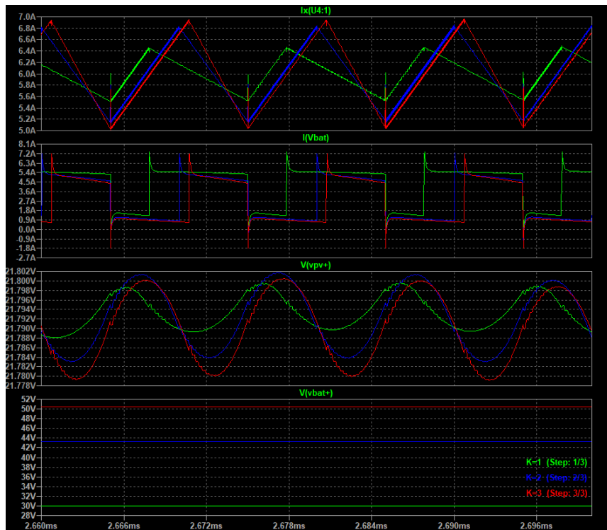
Figure 4.9: 3 stages of charge waveforms in zoomed view.
