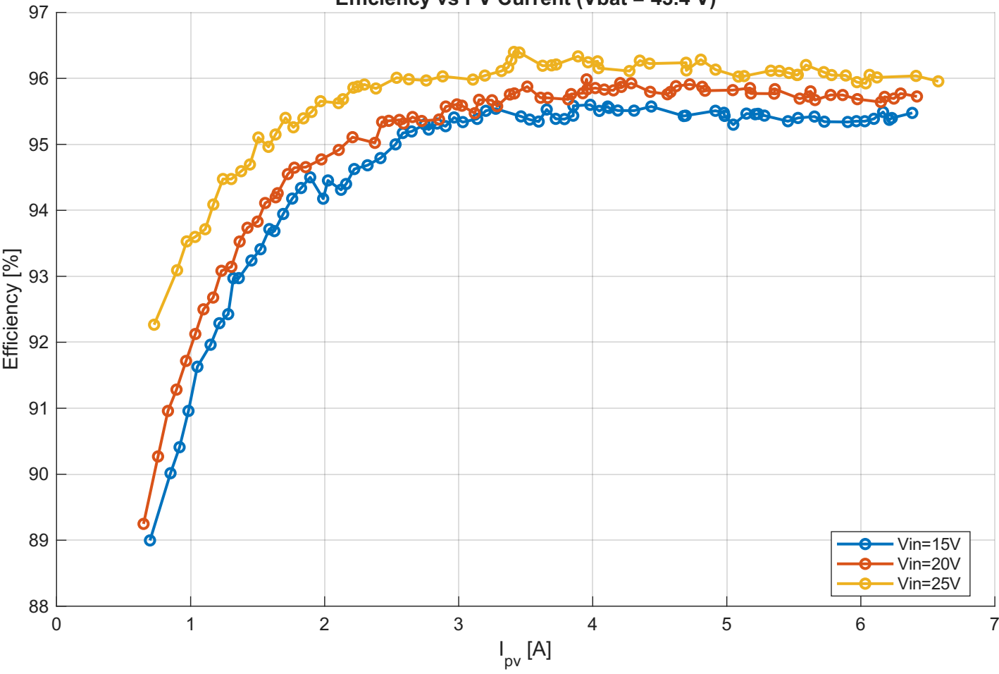
Efficiency vs PV Current (Vbat = 43.4 V)
