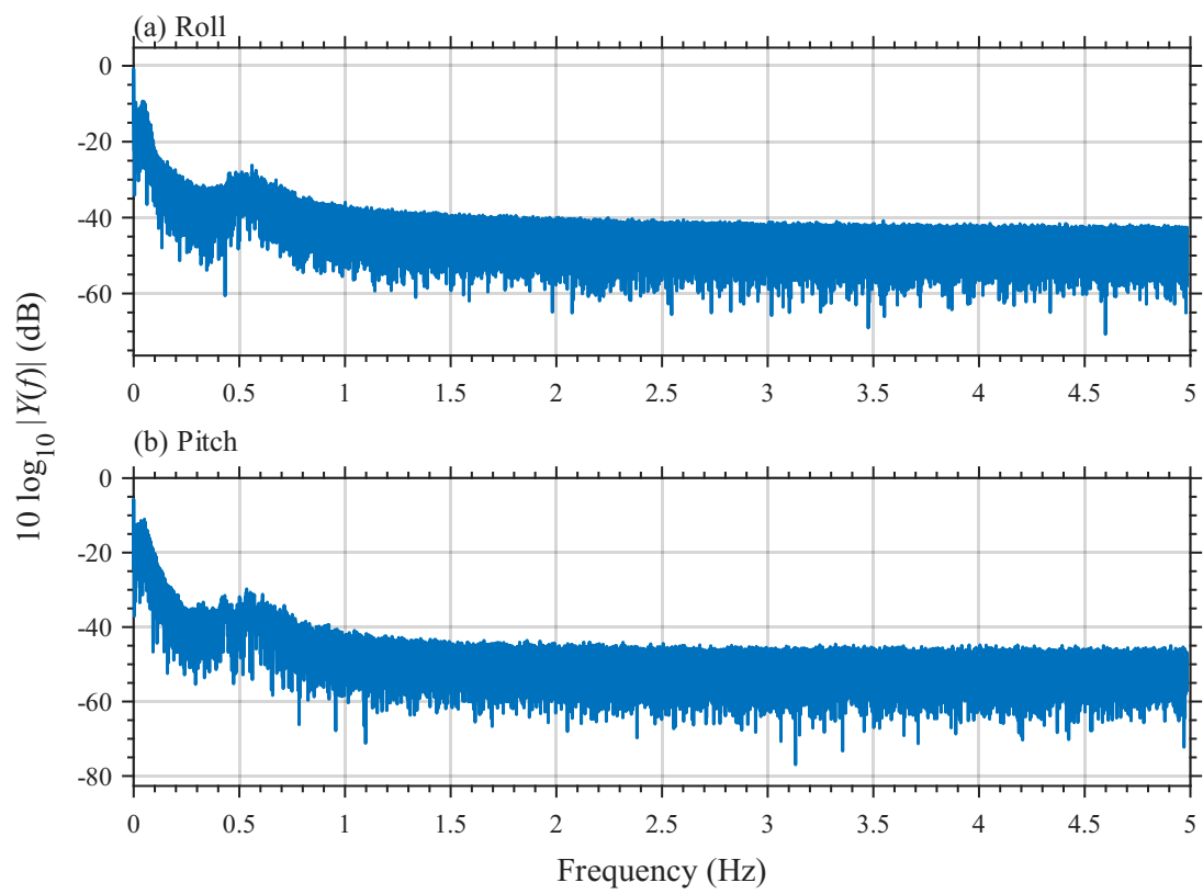
Figure 2.6: Measured oscillations from sg01.
