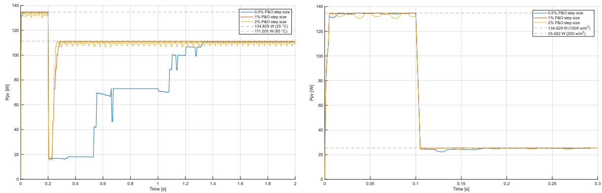
Figure 5.10: Power response for different P&O step sizes during a temperature variation from 25^\circ\text{C} to 85^\circ\text{C} .
