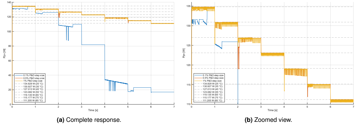
Figure 5.9: Power response for different P&O step sizes during a temperature variation of 10^\circ\text{C} per second.
