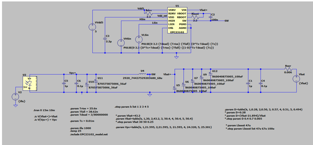
Figure 4.6: Simulation circuit schematic.
