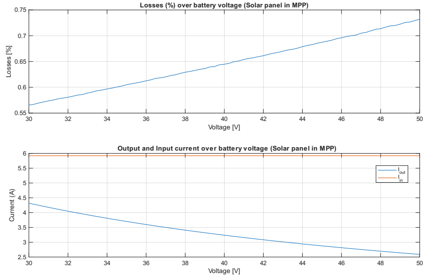
Figure 4.7: Battery voltage sweep simulation results.
