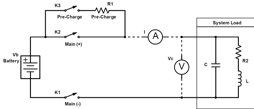
Figure 4.9: Typical precharge circuit [10].
