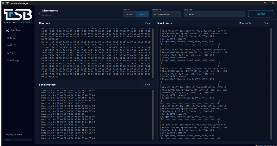
Figure 4.11: Debug page.
