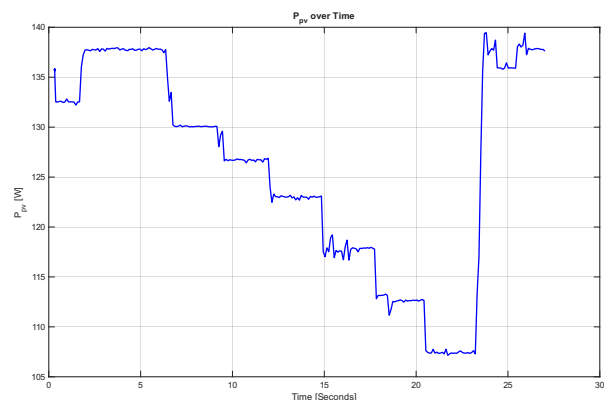
Figure 6.14: Power response for the "Temperature staircase" test.
