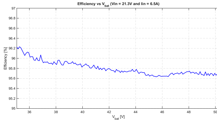
Figure 6.12: Converter efficiency over output voltage.
