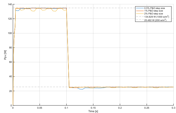
Figure 5.11: Power response for different P&O step sizes during a Irradiance variation from 1000 W/m 2 to 200 W/m 2 .
