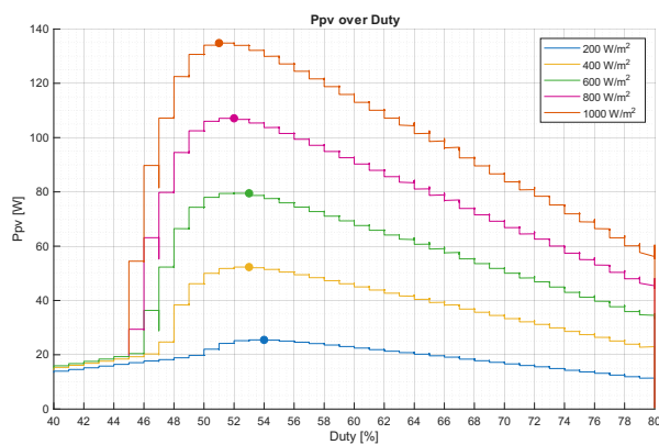
Figure 5.7: Duty cycle sweep with different values of irradiance.
