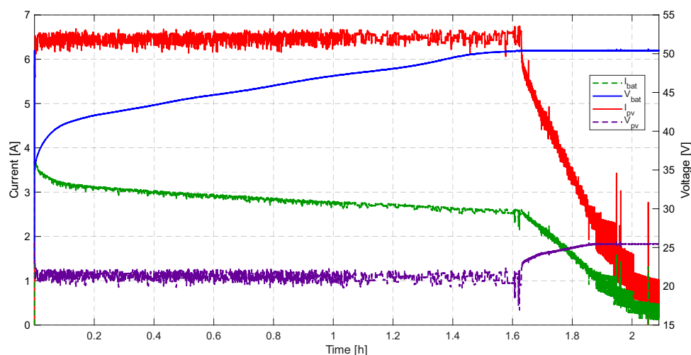
Figure 6.15: Full battery charge in laboratory.
