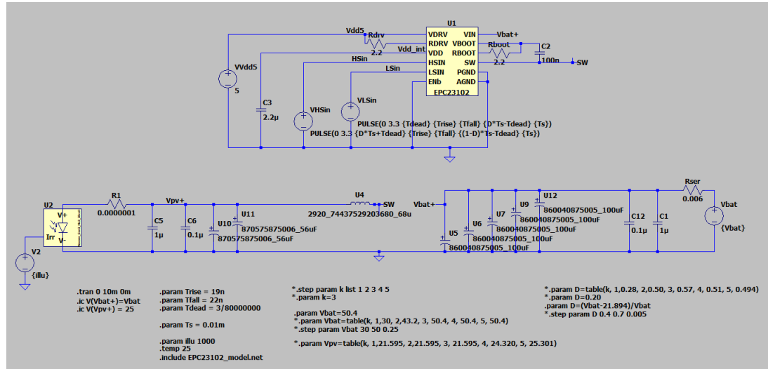
Figure 5.3: Simulation circuit schematic.
