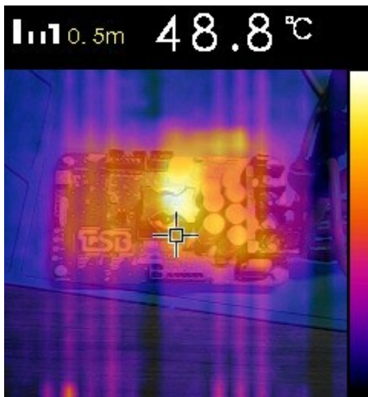
Figure 6.7: Front side thermal image.
