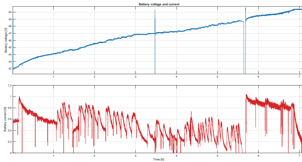
Figure 6.16: Battery charging test. Voltage and current curve.
