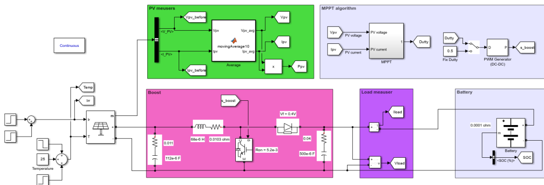
Figure 5.6: MATLAB Simulink MPPT simulation model.
