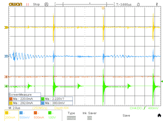
Figure 6.6: Measured waveforms after adding nine additional 1 μF ceramic capacitors.
