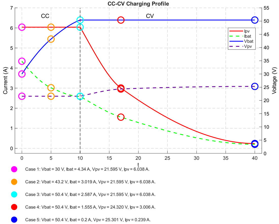
Figure 5.2: CC-CV charge characteristics and analysis point selection.
