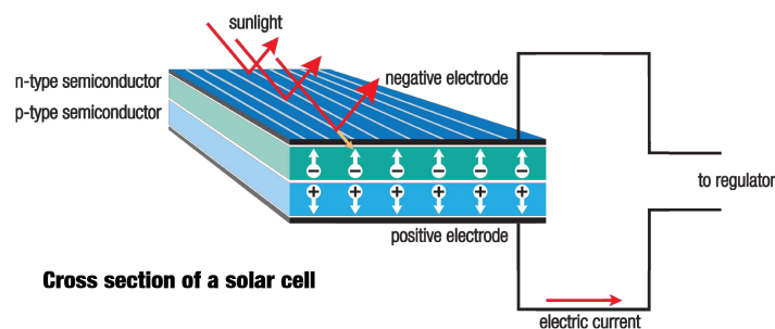
Figure 3.1: Principle of operation of a solar panel [2].
