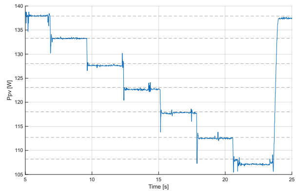
Figure 6.14: Power response for the "Temperature staircase" test.
