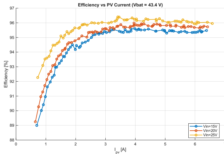
Figure 6.11: Converter efficiency over different input currents and voltages.
