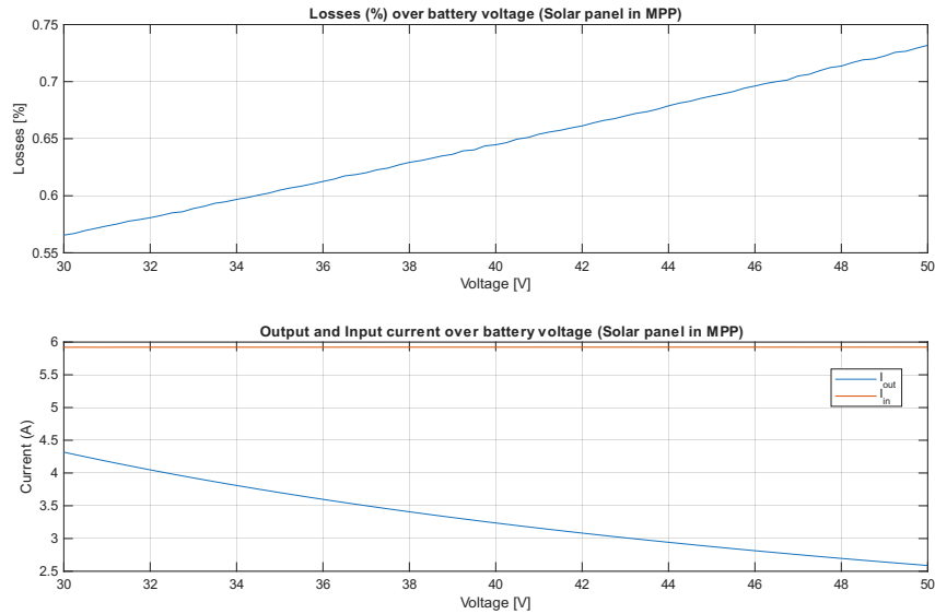
Figure 5.4: Battery voltage sweep simulation results.
