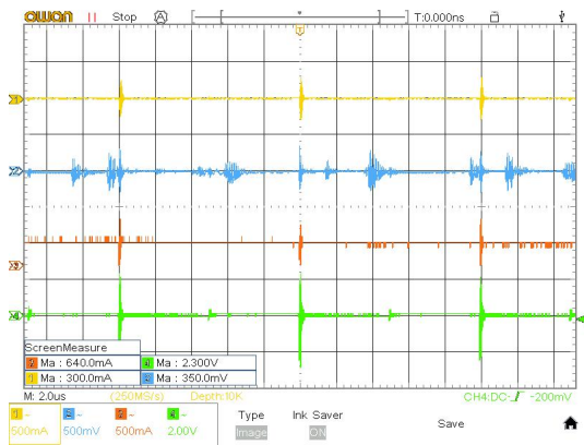
Figure 6.5: Measured waveforms after adding nine additional 1 μF ceramic capacitors.
