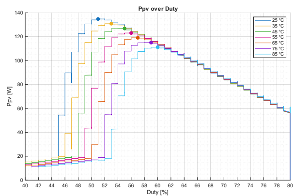
Figure 5.8: Duty cycle sweep with different values of temperature.
