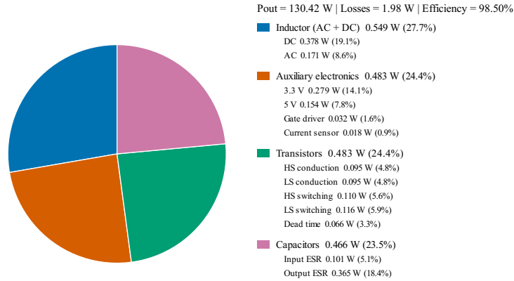
Figure 5.5: Prototype analytical power loss distribution at Case 2.
