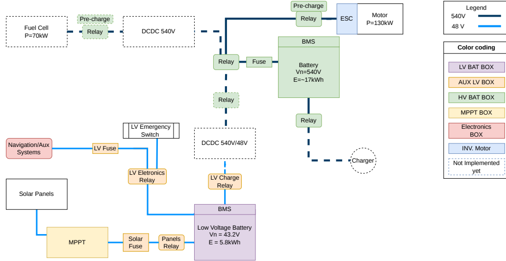
Figure 2.1: Simplified electrical schematic of SG01.
