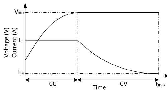
Figure 3.11: Charging profile of CC/CV [7].
