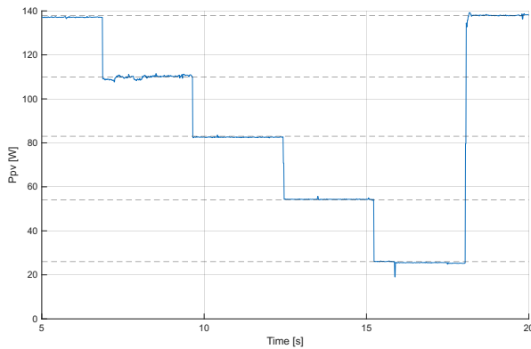
Figure 6.13: Power response for the "Irradiance staircase" test.
