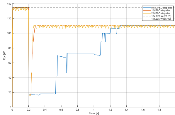
Figure 5.10: Power response for different P&O step sizes during a temperature variation from 25°C to 85°C.
