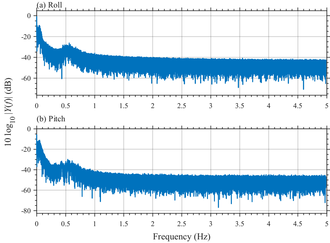
Figure 2.6: Measured oscillations from SG01.
