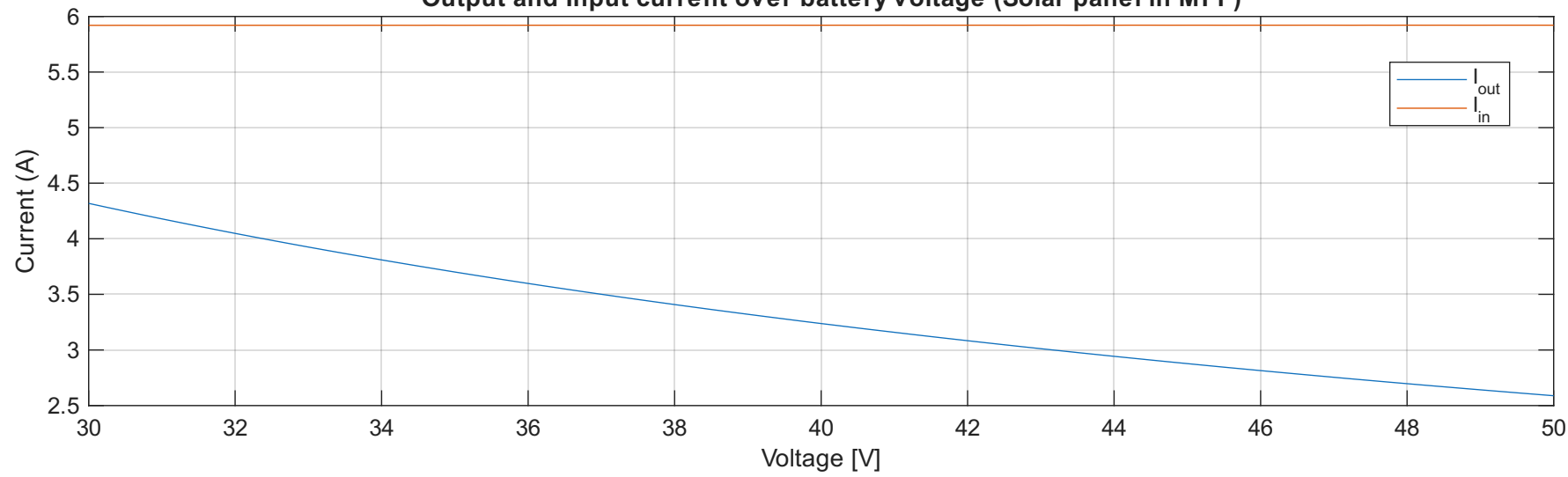
Output and Input current over battery voltage (Solar panel in MPP)
