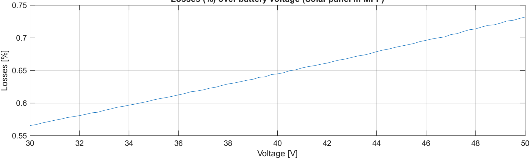
Losses (%) over battery voltage (Solar panel in MPP)
