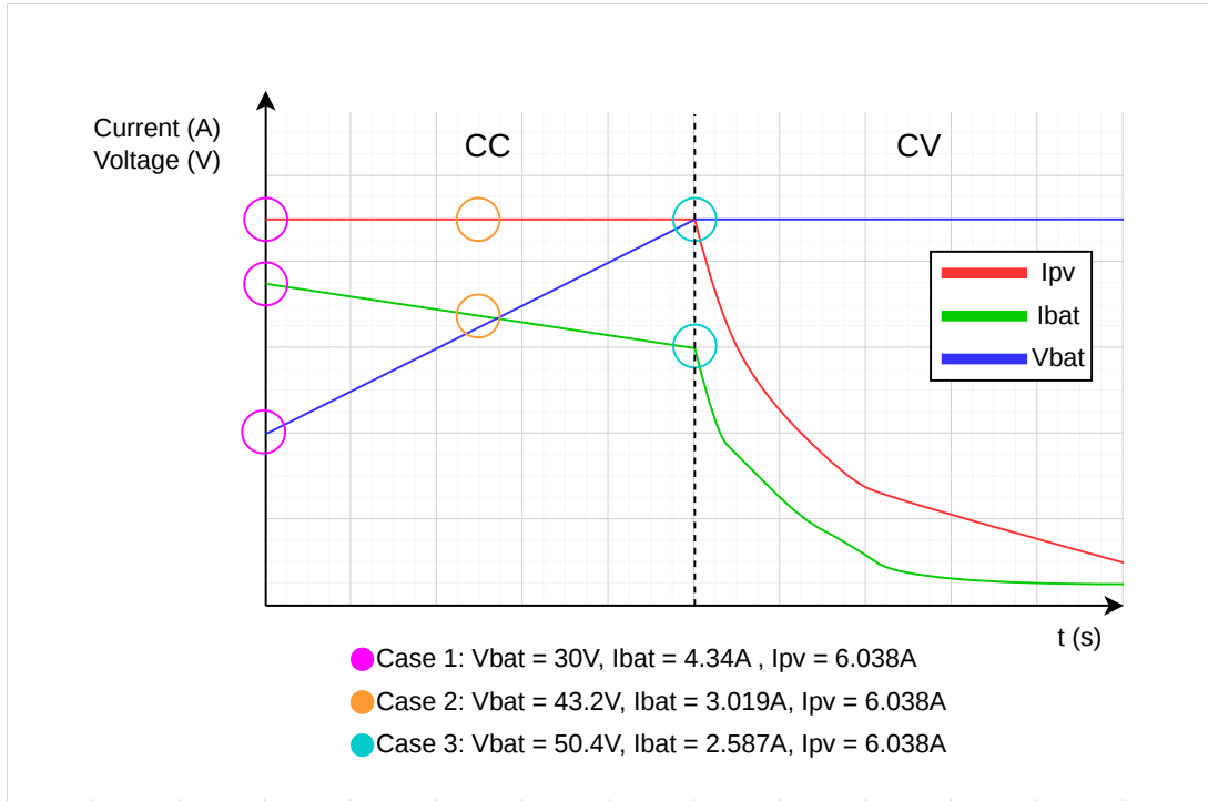
Figure 5.2: CC-CV charge characteristics and case selection.
