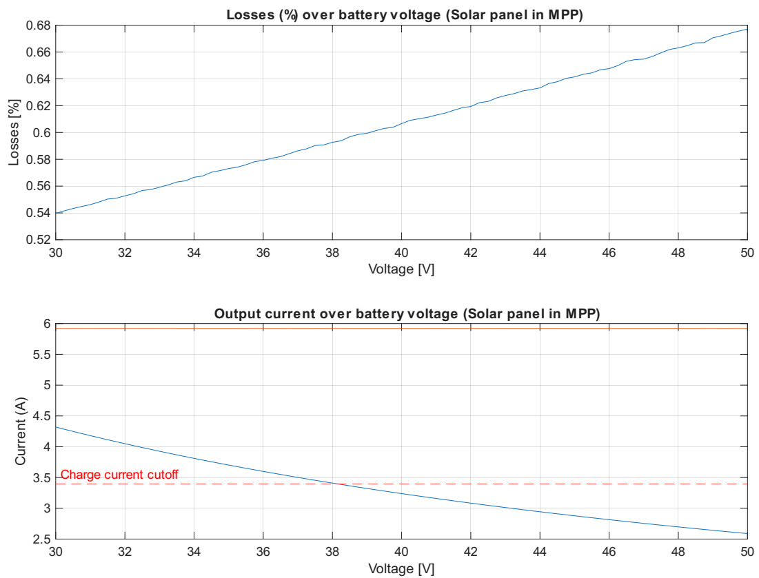
Figure 5.4: Battery voltage sweep simulation results.
