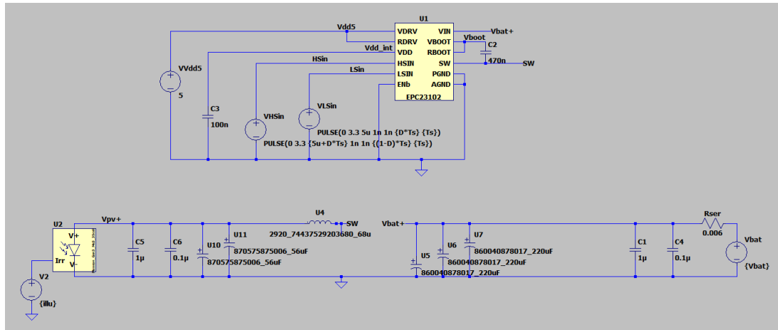
Figure 5.3: Simulation circuit diagram.
