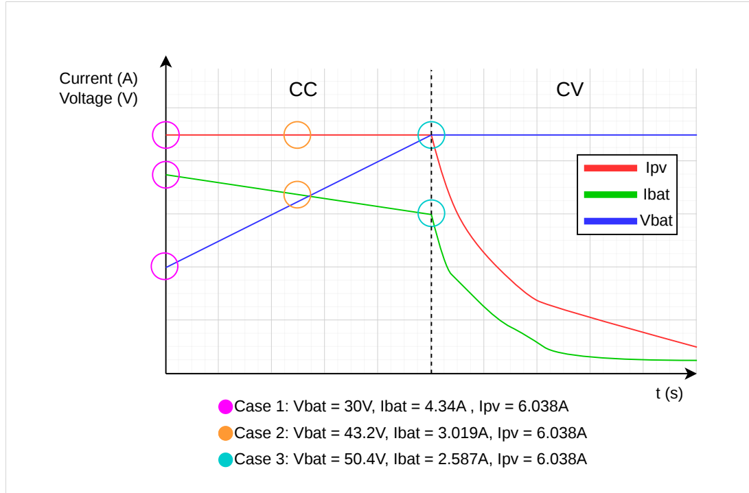
Figure 4.6: CC-CV charge characteristics and case selection.
