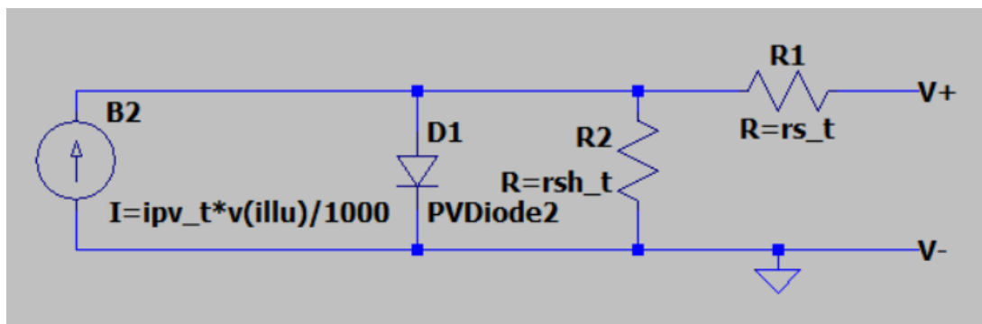
Figure 4.5: Solar panel model diagram (1M5P configuration).
