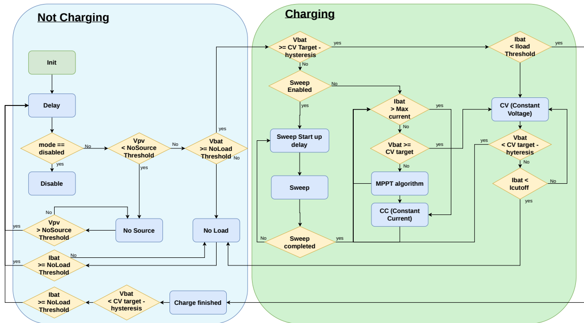
Figure 4.6: Charging state machine state.
