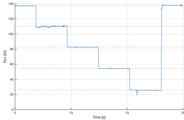
Figure 6.13: Power response for the "Irradiance staircase" test.
