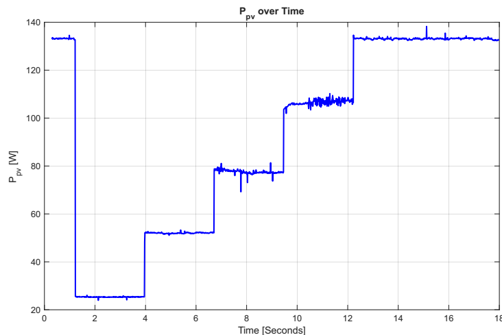
Figure 6.10: PV Power over time with steps of 200 W/m 2 , from 200 to 1000 W/m 2 .
