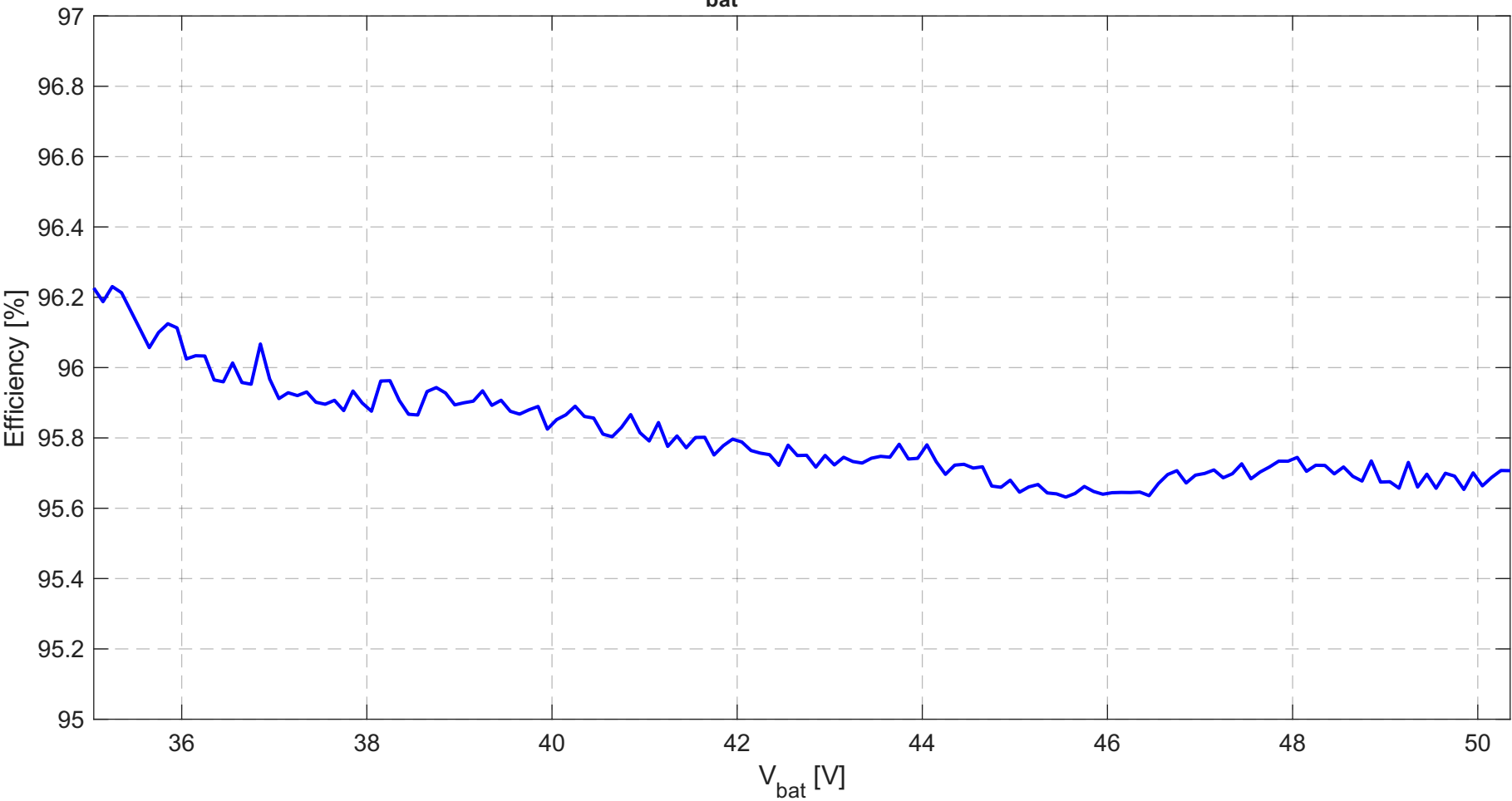
Efficiency vs V_{bat} ( V_{in} = 21.3V and I_{in} = 6.5A )
