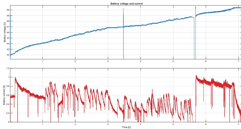
Figure 6.14: Battery charging test. Voltage and current curve.
