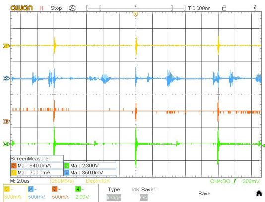
Figure 6.5: Measured waveforms after adding nine additional 1 \mu F ceramic capacitors.
