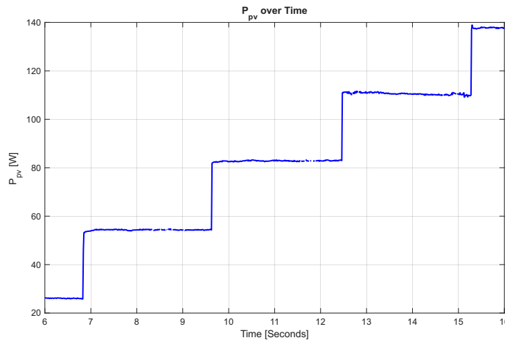
Figure 6.13: PV Power over time with steps of 200 \text{ W/m}^2 , from 200 \text{ W/m}^2 to 1000 \text{ W/m}^2 .
