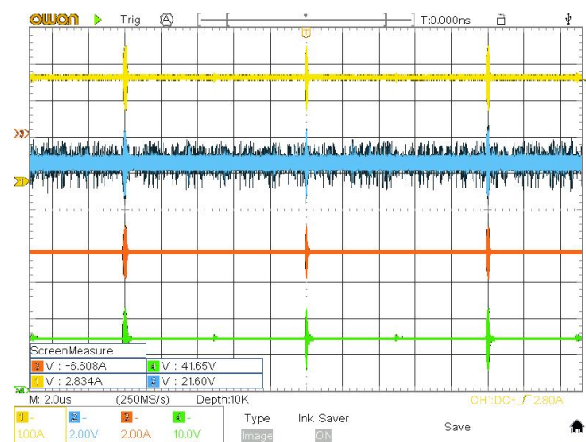
Figure 5.3: Measured waveforms before adding the additional ceramic capacitors.
