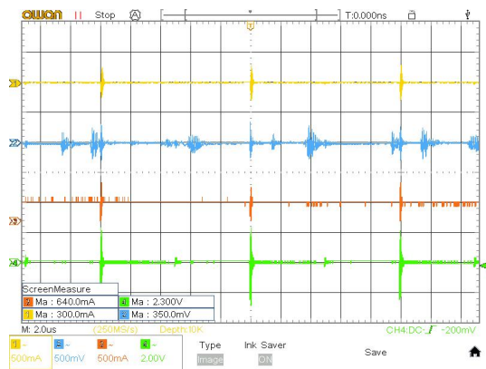
Figure 5.4: Measured waveforms after adding nine additional 1\ \mu\text{F} ceramic capacitors.
