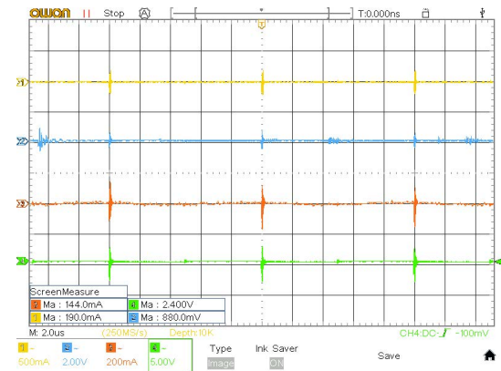
Figure 5.5: Measured waveforms after adding nine additional 1\ \mu\text{F} ceramic capacitors.
