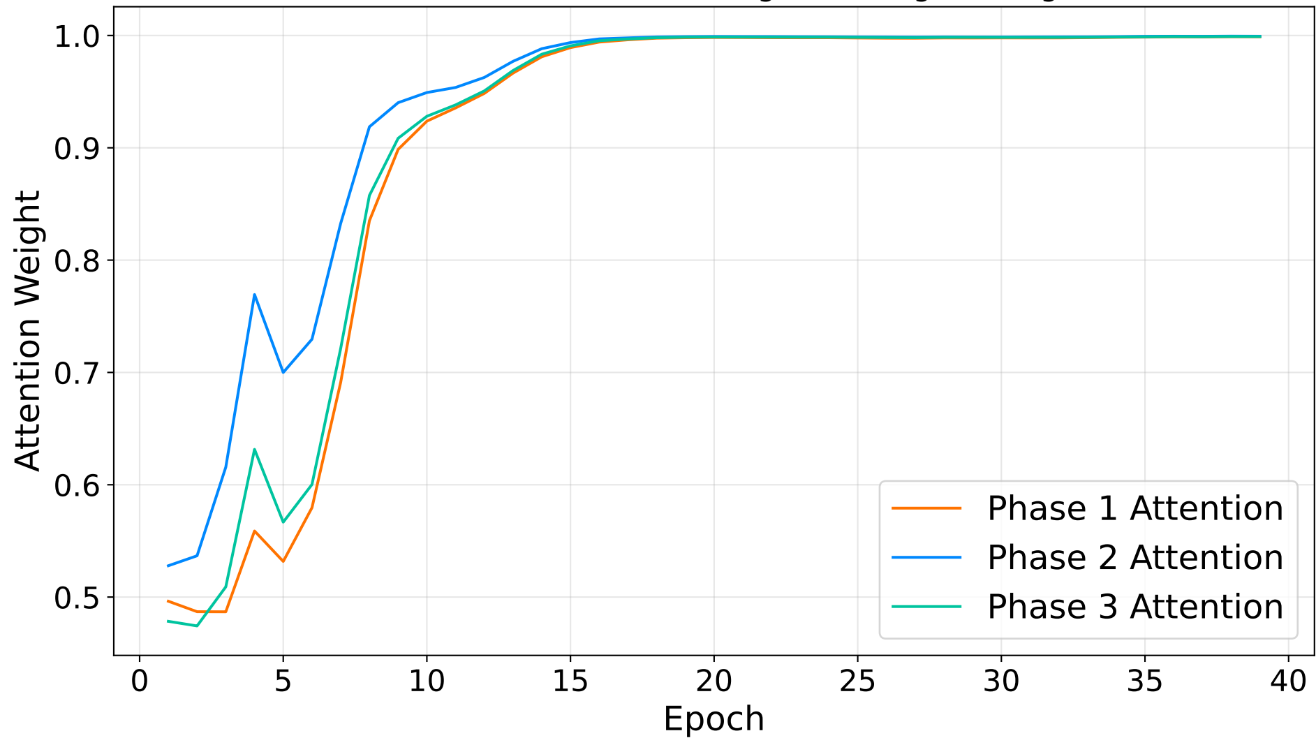
Evolution of Attention Weights During Training
