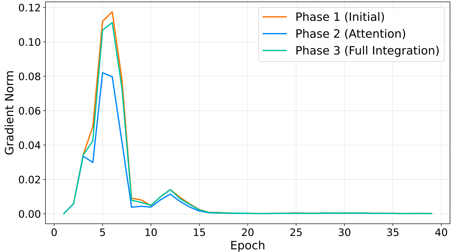
Evolution of Gradient Norms During Training
