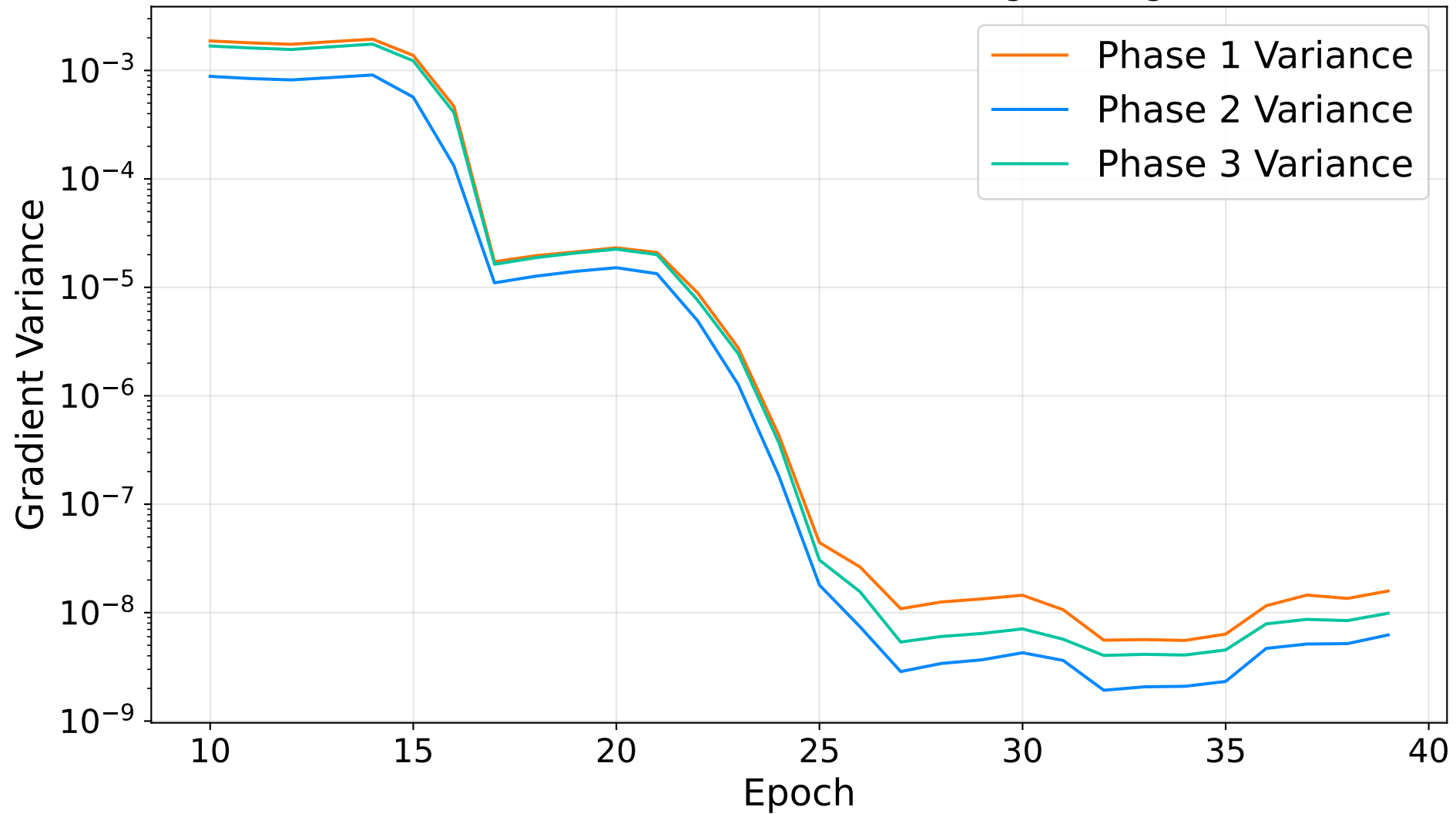
Gradient Variance Reduction During Training
