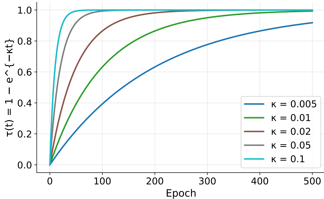
Curriculum Schedule \tau(t) (Theorem 3: schedule rate \kappa )
