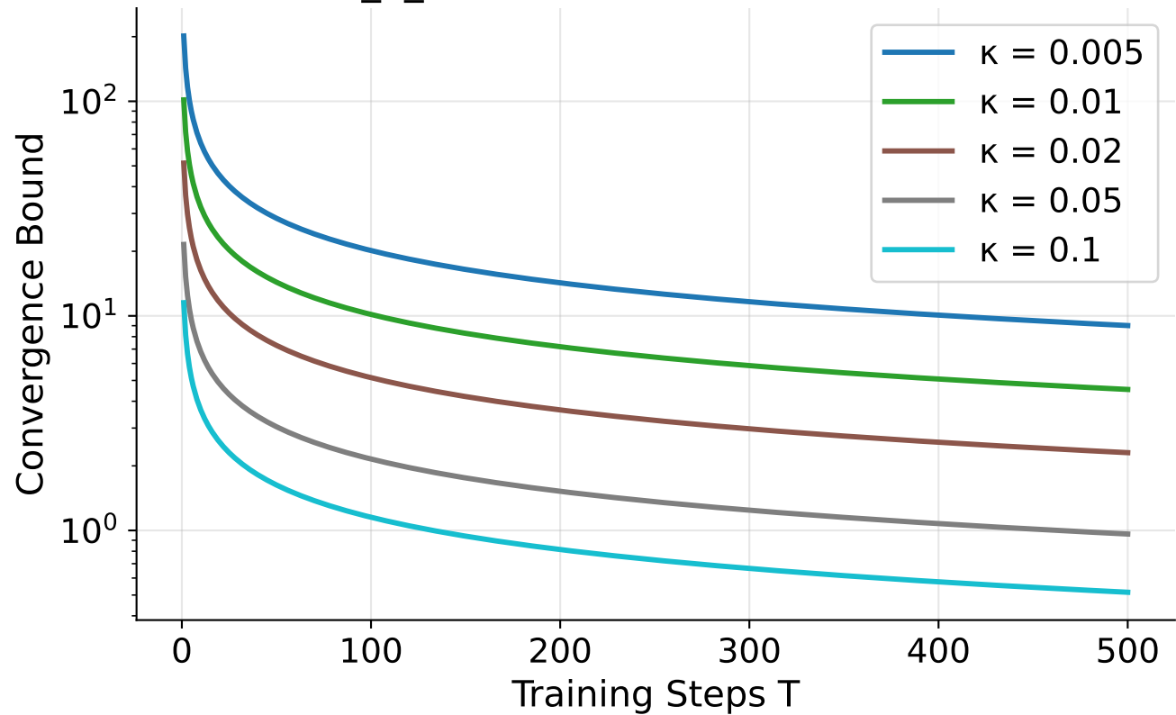
Theoretical Convergence Bound E[R(f_{\theta_T}) - R^*] \leq O(1/\sqrt{T}) (Theorem 3)
