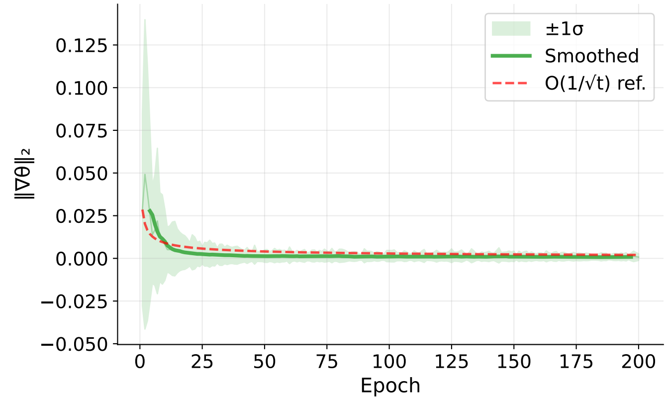
Phase-3 (Embed) (raw \pm \sigma + smoothed)
