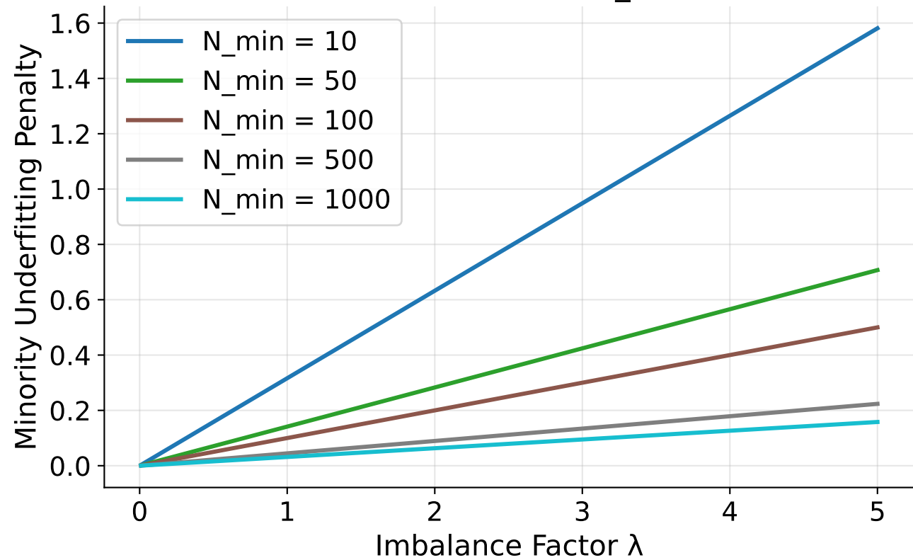
Enact Phase Minority Penalty vs \lambda (Theorem 2: \propto \lambda/\sqrt{N_{\min}} )
