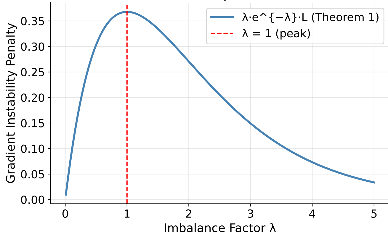
Engage Phase Gradient Penalty vs \lambda (Theorem 1: decays as \lambda \cdot e^{-\lambda} )
