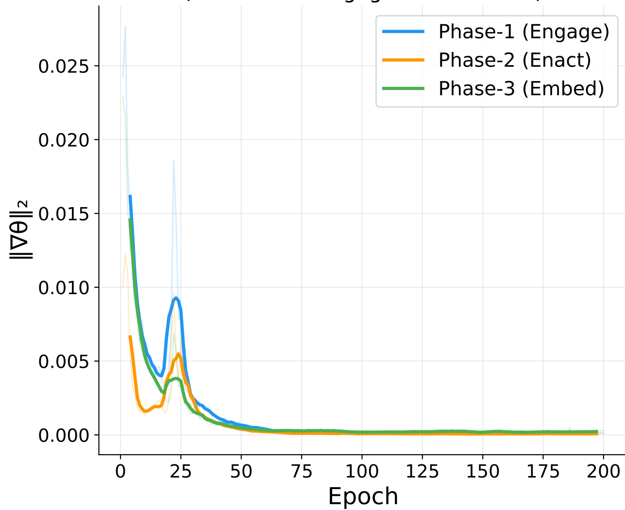
Gradient Norm per Phase (Theorem 1: Engage bounds \lambda e^{-L} )
