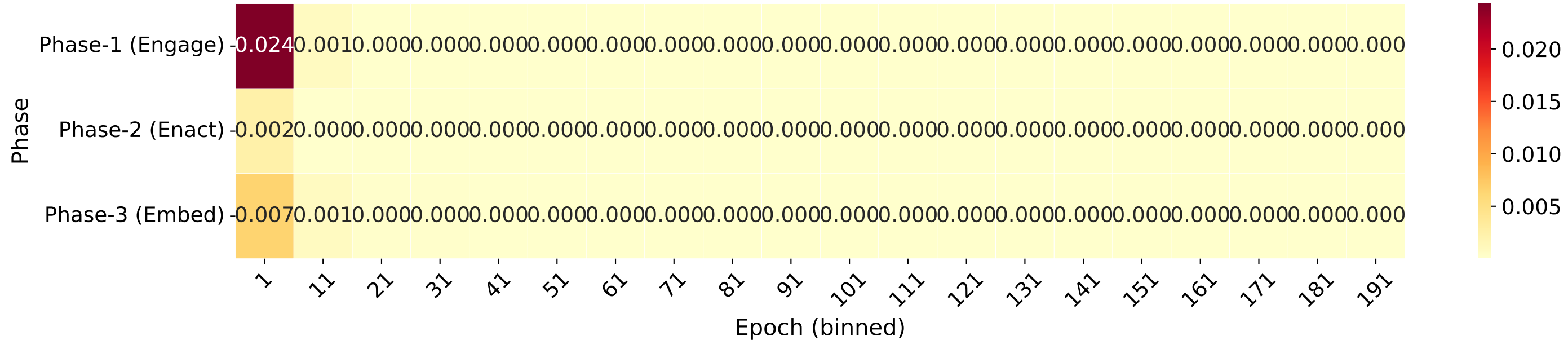
Gradient Variance Heatmap per Phase (Validates Theorem 1: \text{Var}[\nabla] \leq L^2/N )
