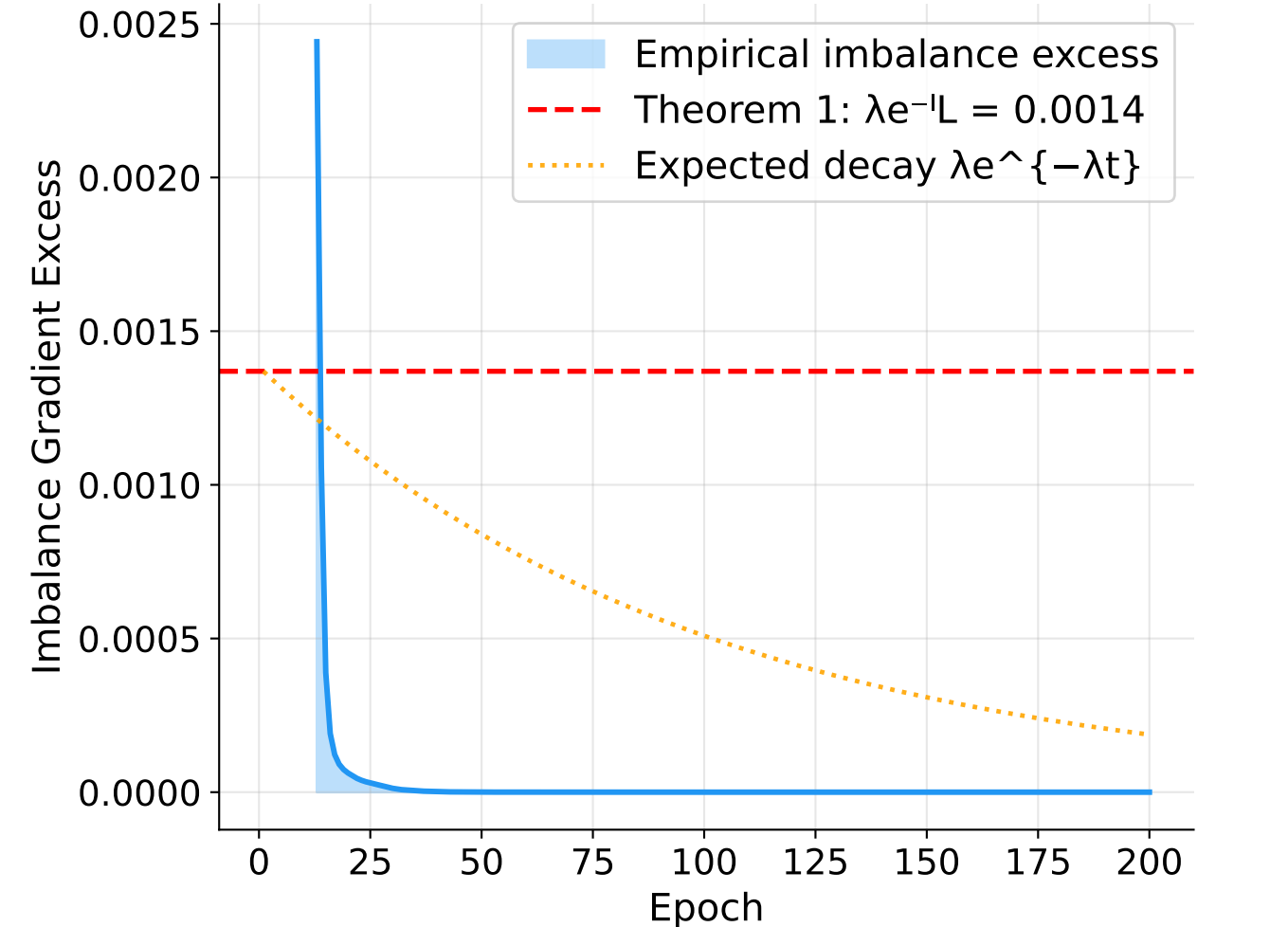
Imbalance Penalty Validation Engage phase excess \leq \lambda e^{-L} (Theorem 1 term 3)
