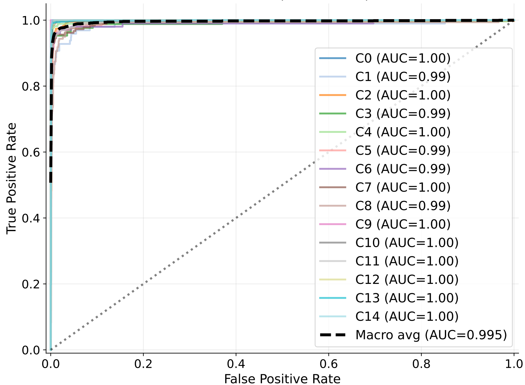
ROC Curves (One-vs-Rest)
