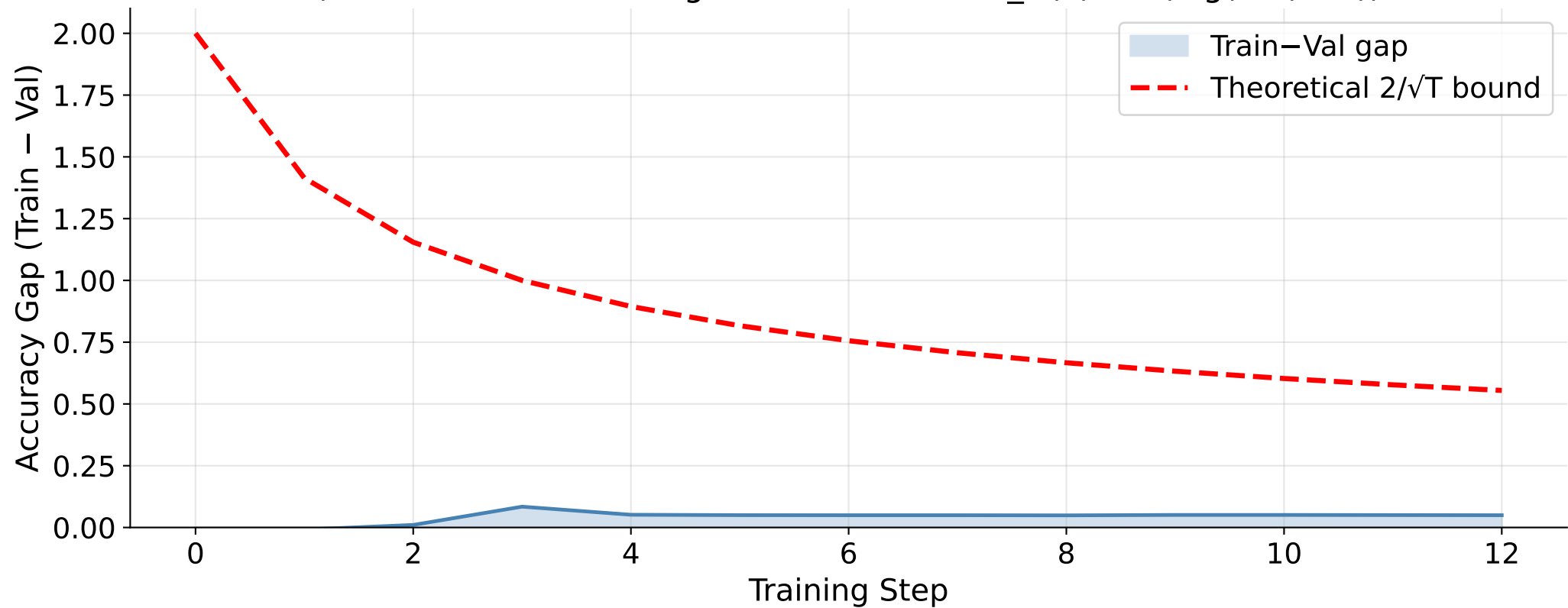
Generalisation Gap as Rademacher Proxy (Validates Theorem 2: \text{generalisation} \leq 2R_N(F) + \sqrt{(\log(1/\delta)/2N)} )
