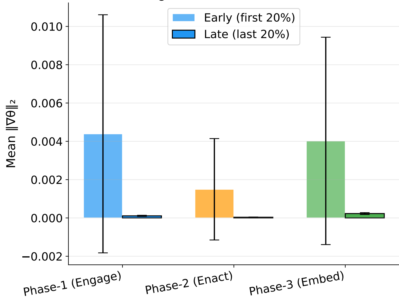
Early vs Late Gradient Norms (Convergence: norms should decrease)
