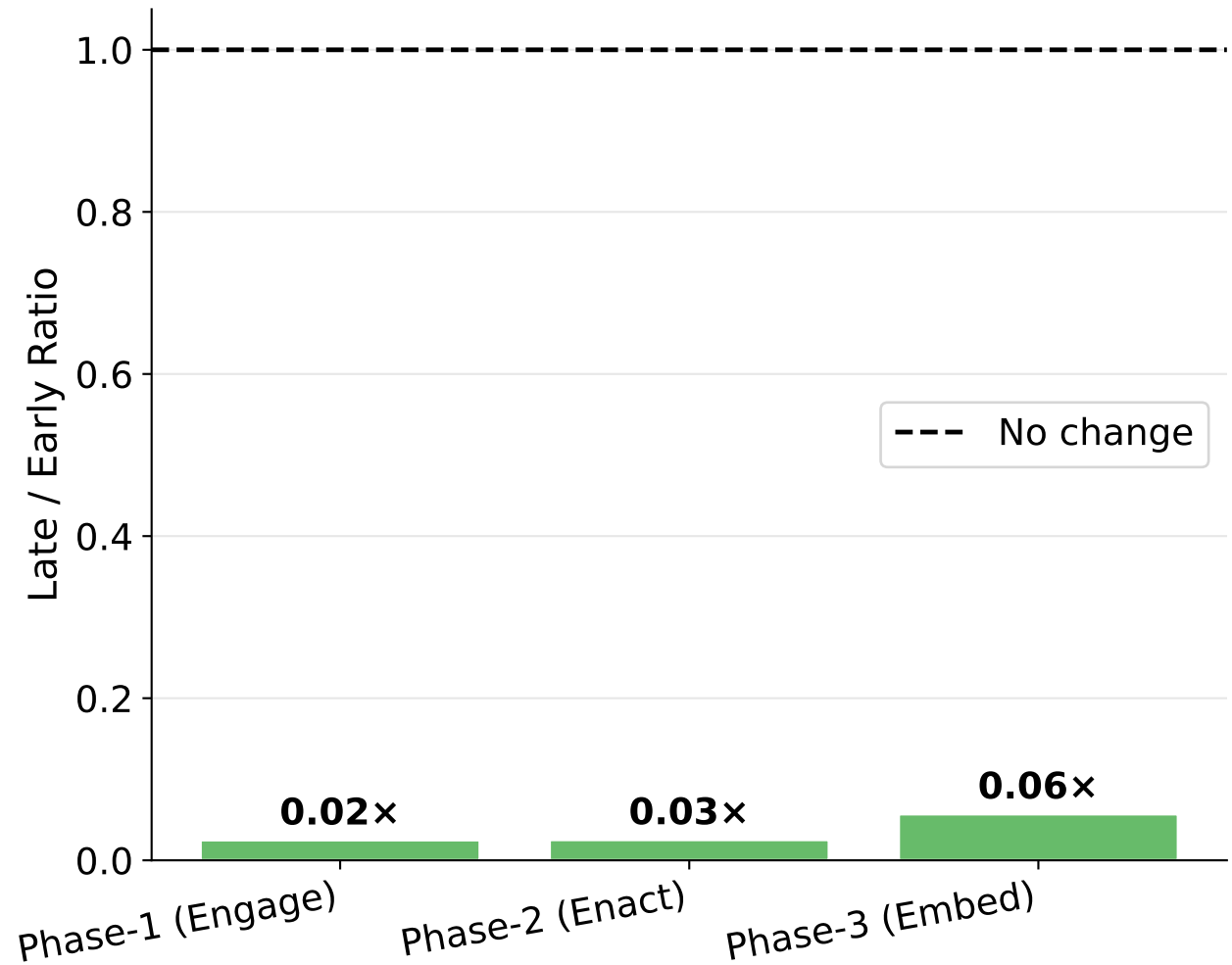
Gradient Reduction Ratio ( < 1.0 = stabilised)
