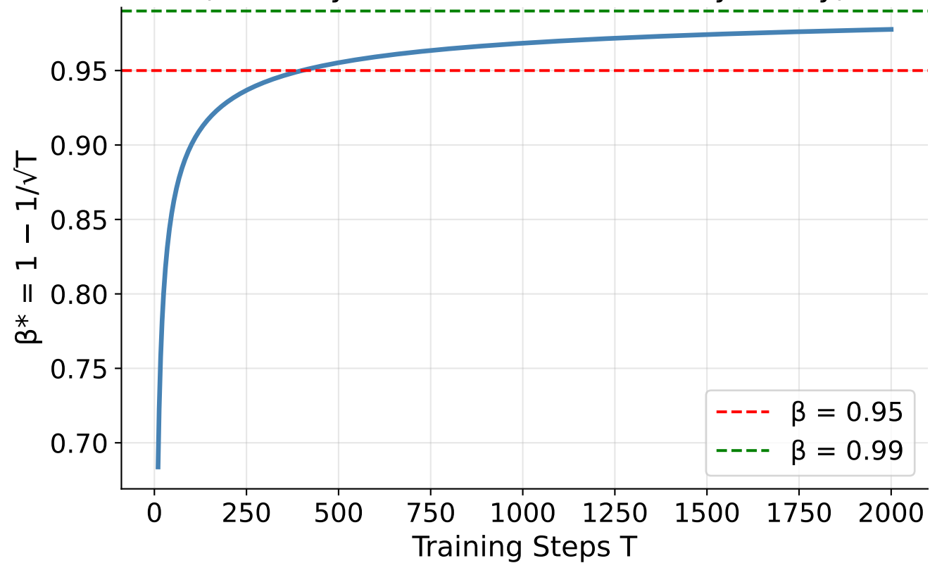
Optimal Memory Forgetting Factor \beta^* (Corollary 4: Embed Phase Memory Decay)
