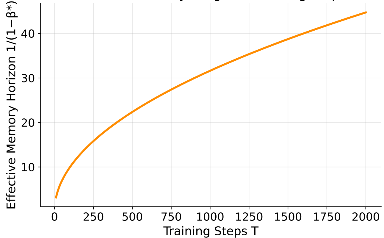
Effective Memory Length vs Training Steps
