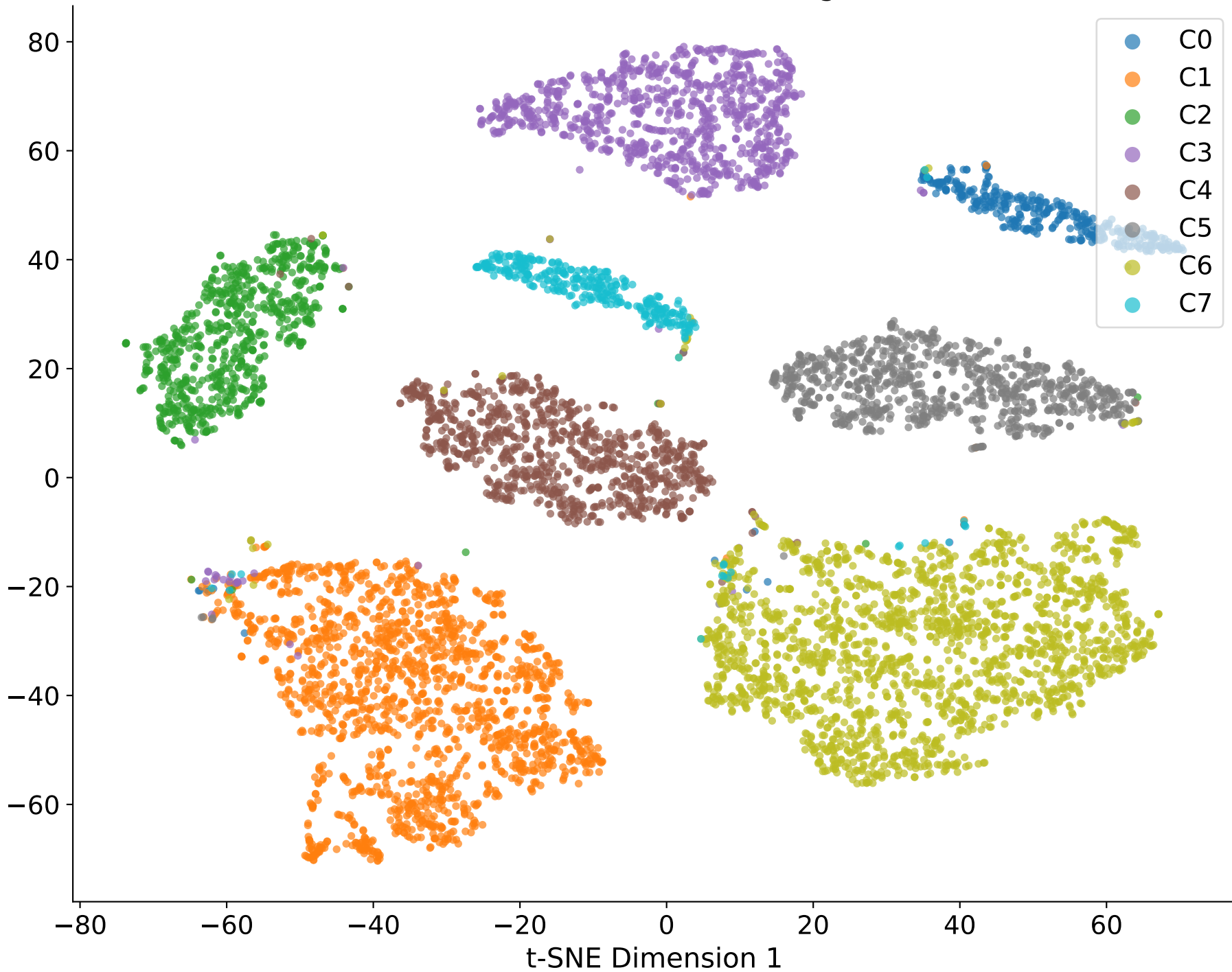
t-SNE of Node Embeddings
