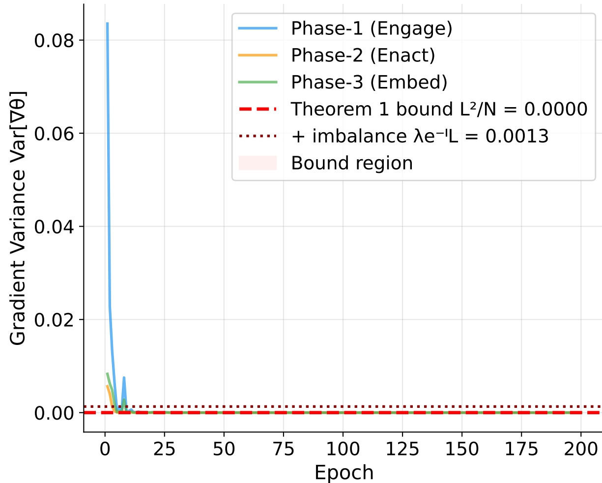
Empirical Variance vs Theorem 1 Bound \text{Var}[\nabla] \leq L^2/N
