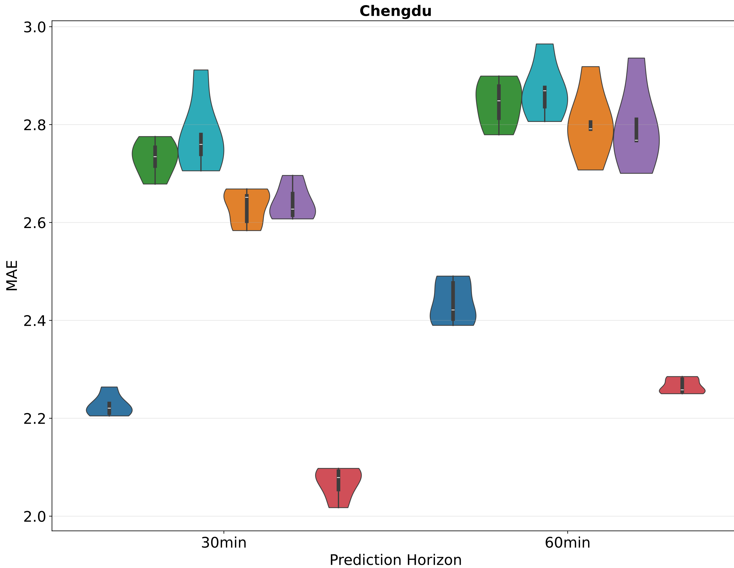
Violin Plots -- Chengdu & Shenzhen (30-min & 60-min horizons) MCPST vs Top-5 Transfer & Prompt-Based Models | MAE across 5 runs
