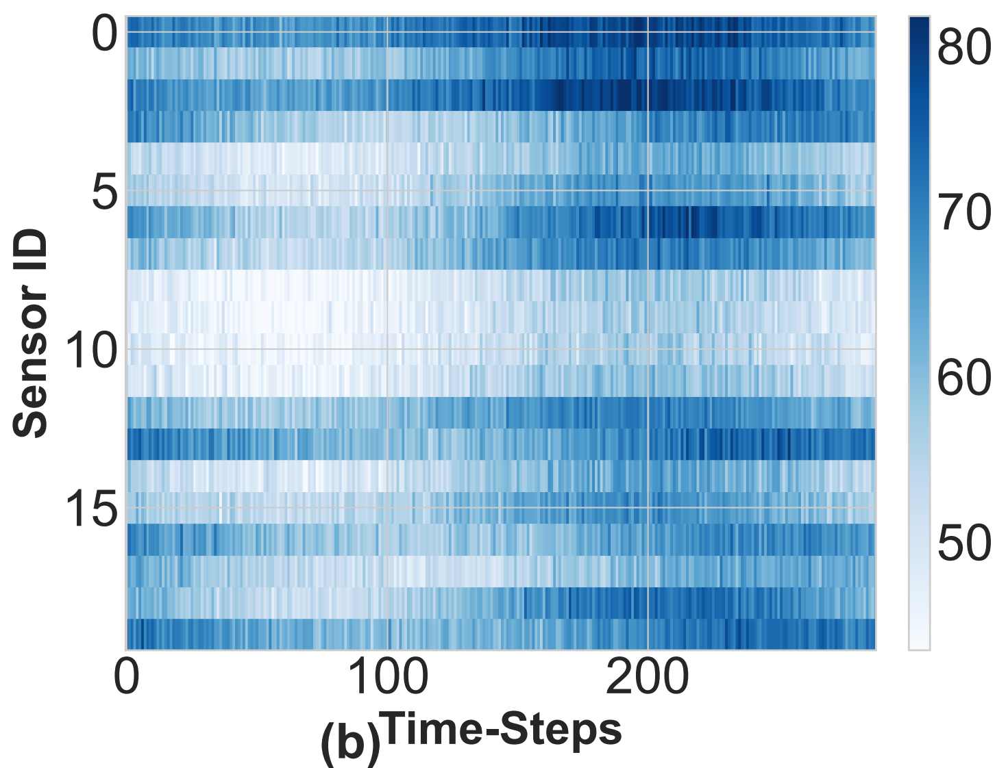
MCPST Predictions MAE: 1.565
