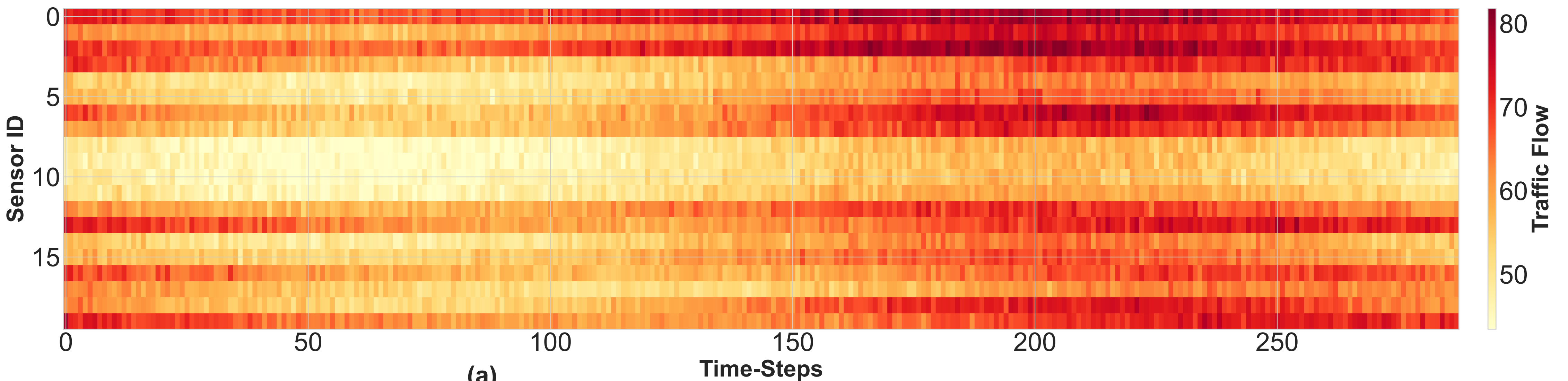
MCPST Predictions MAE: 1.565
