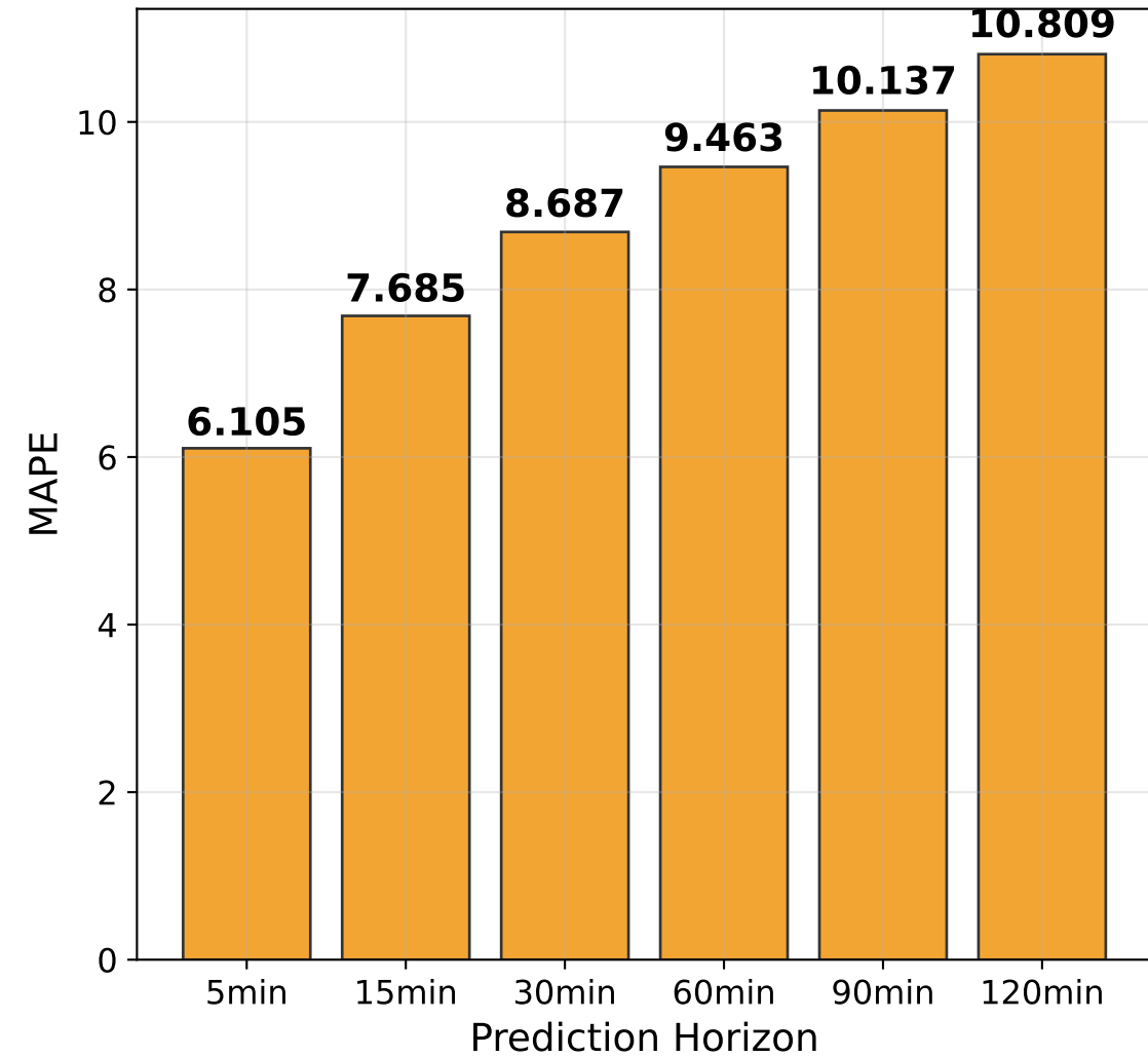
MAPE Across Horizons
