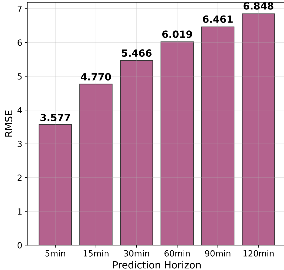
RMSE Across Horizons
