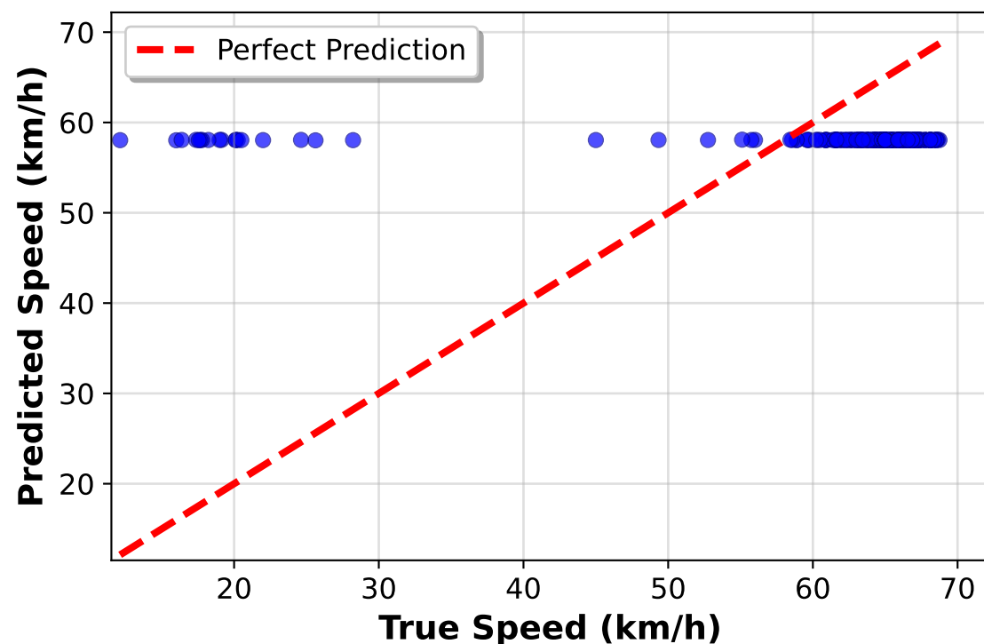
Node 1, Horizon 1 MAE: 9.27, RMSE: 12.93 R 2 : -0.040, MAPE: 26.2% Bias: -2.52
