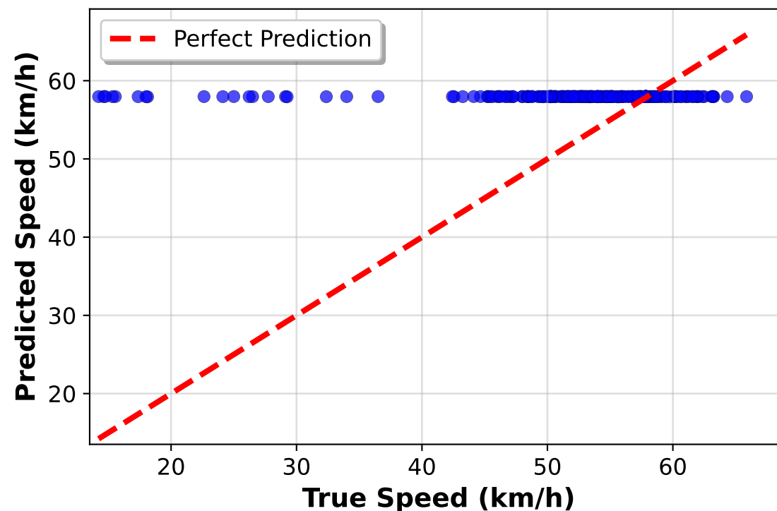
Node 2, Horizon 4 MAE: 7.22, RMSE: 11.55 R 2 : -0.386, MAPE: 22.2% Bias: 6.10
