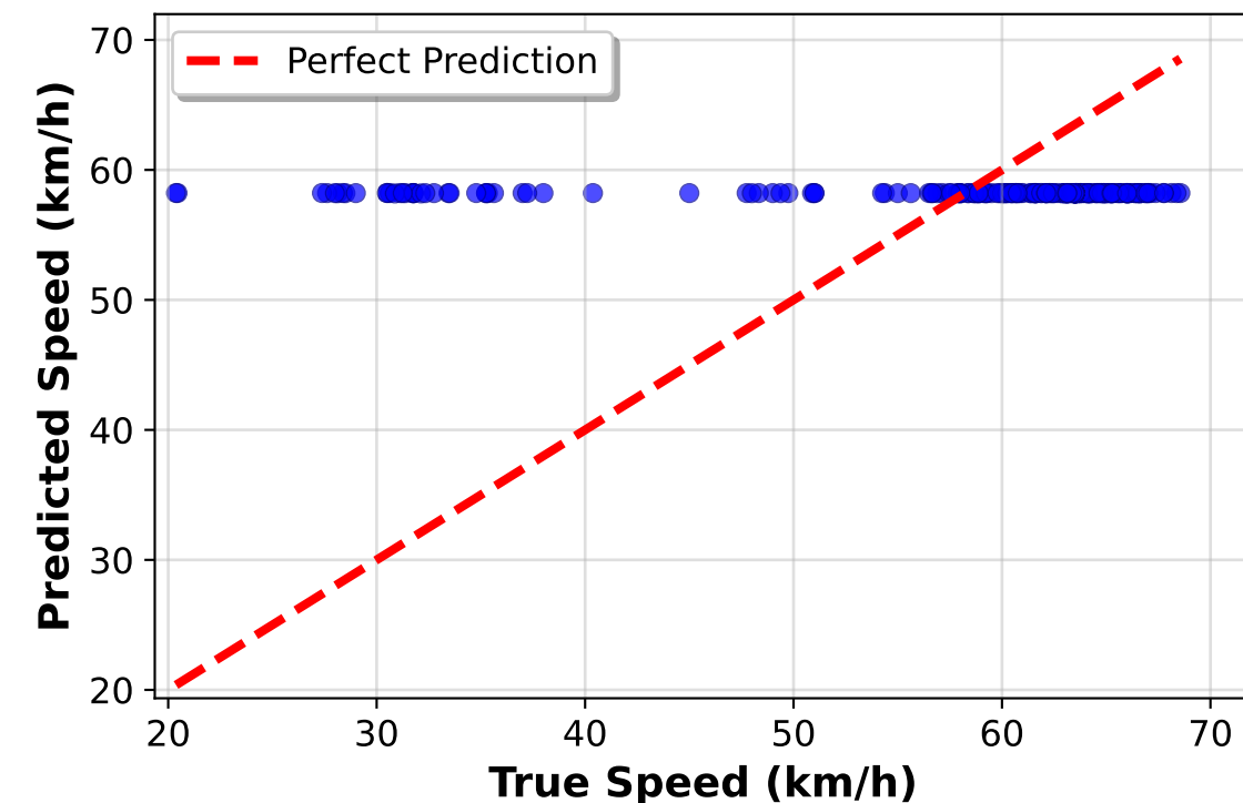
Node 2, Horizon 7 MAE: 8.72, RMSE: 12.16 R 2 : -0.017, MAPE: 21.6% Bias: 1.59
