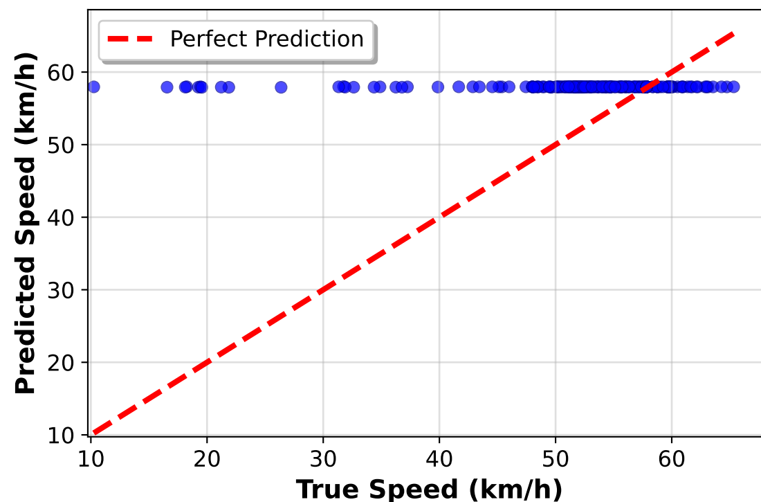
Node 1, Horizon 4 MAE: 7.46, RMSE: 12.12 R 2 : -0.403, MAPE: 24.3% Bias: 6.50
