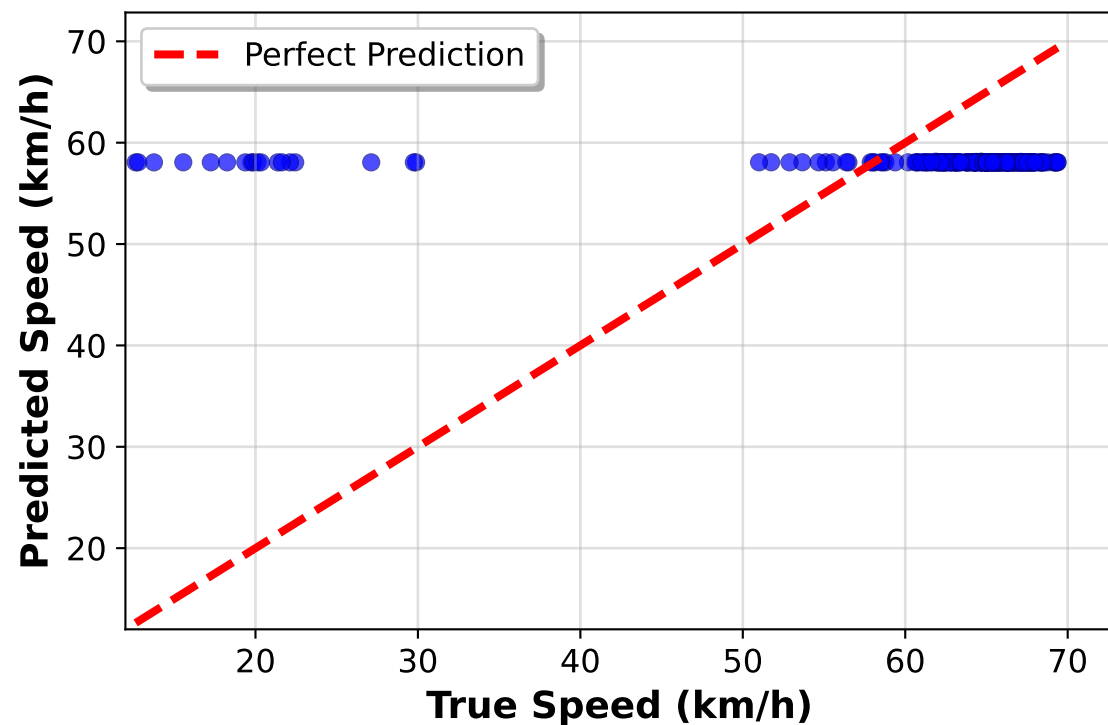
Node 2, Horizon 1 MAE: 9.38, RMSE: 13.12 R 2 : -0.037, MAPE: 27.1% Bias: -2.49
