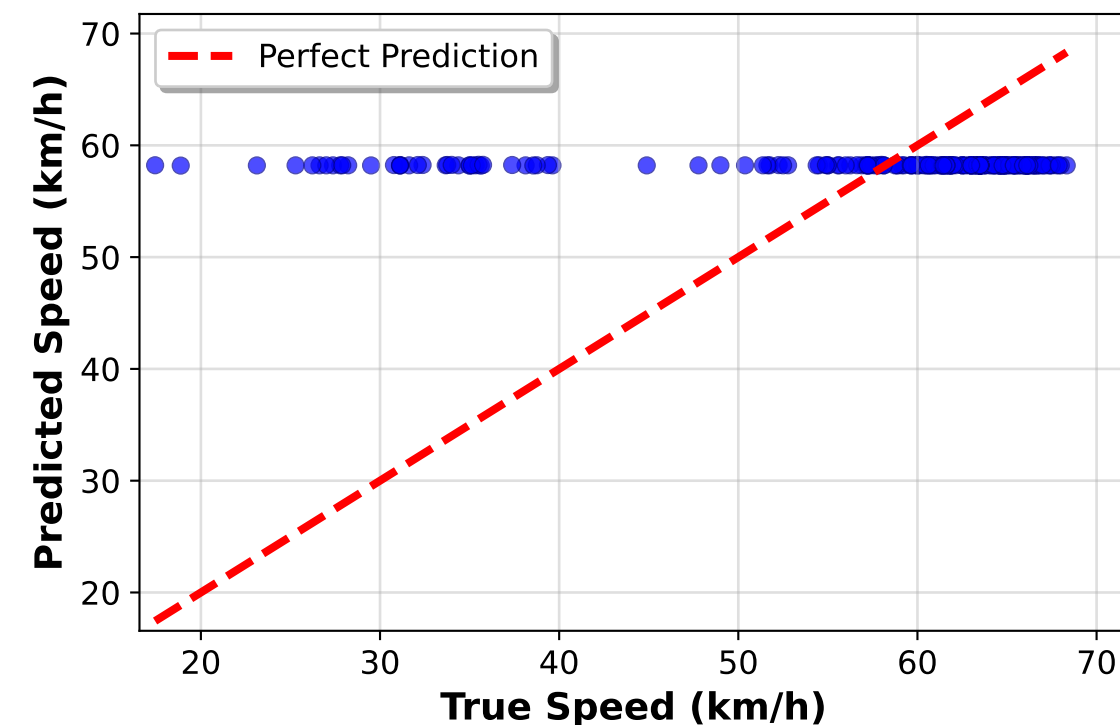
Node 1, Horizon 7 MAE: 8.57, RMSE: 12.10 R 2 : -0.011, MAPE: 21.2% Bias: 1.25
