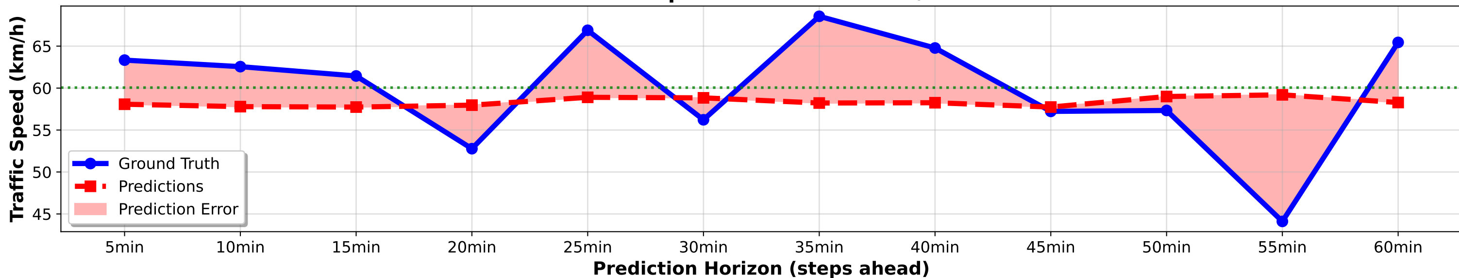
Node 1 - Multi-step Prediction Analysis MAE: 5.90, RMSE: 7.03, Max Error: 15.08, R 2 : -0.126 Mean Speed: 60.1 ± 24.4 km/h
