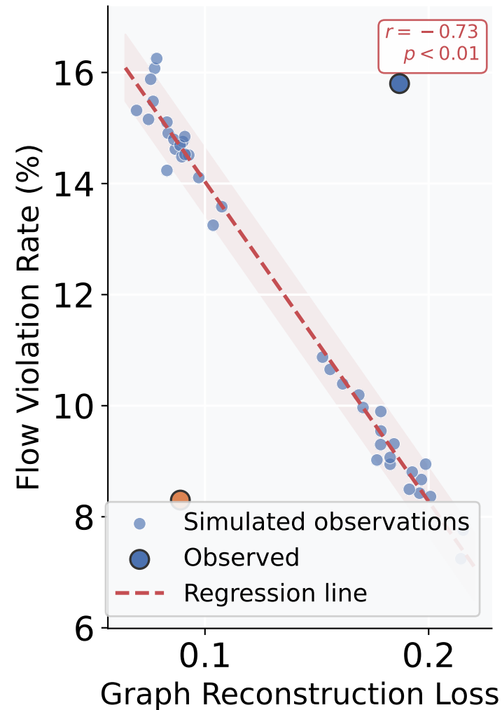
Graph Loss vs Flow Violation (Pearson Correlation)
