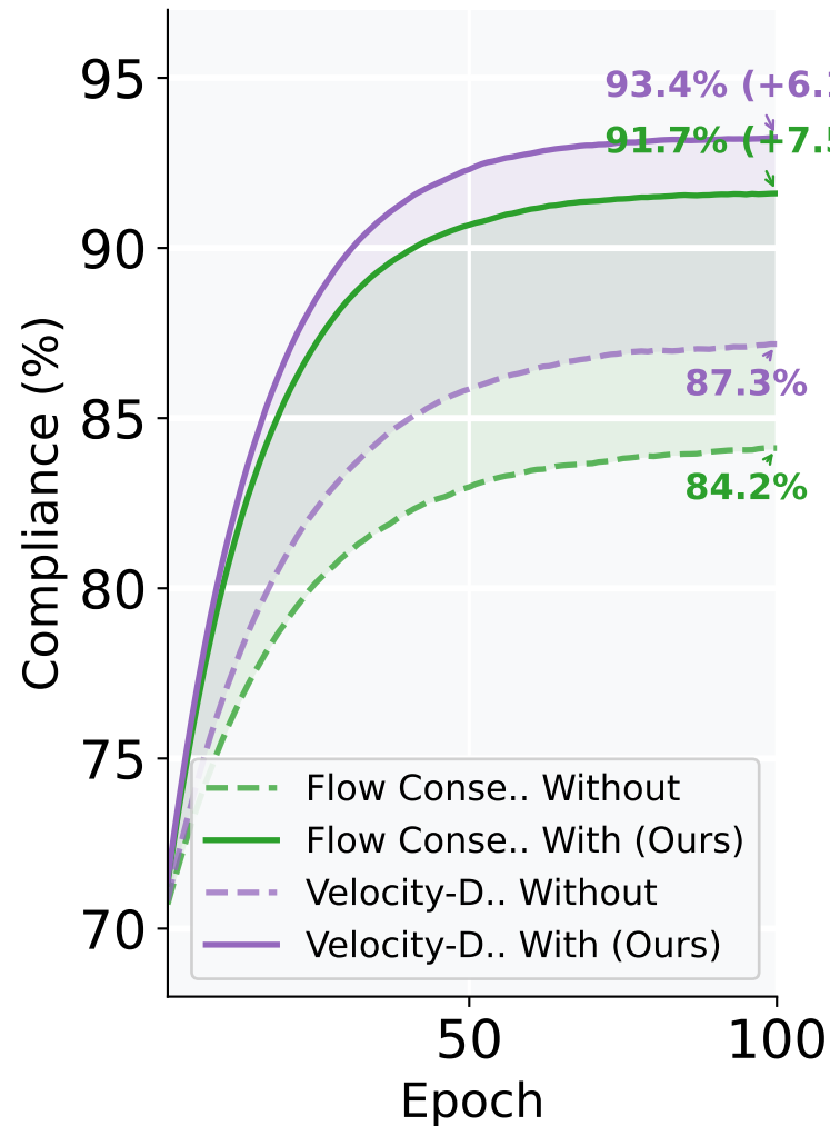
Physical Compliance vs Training Epochs
