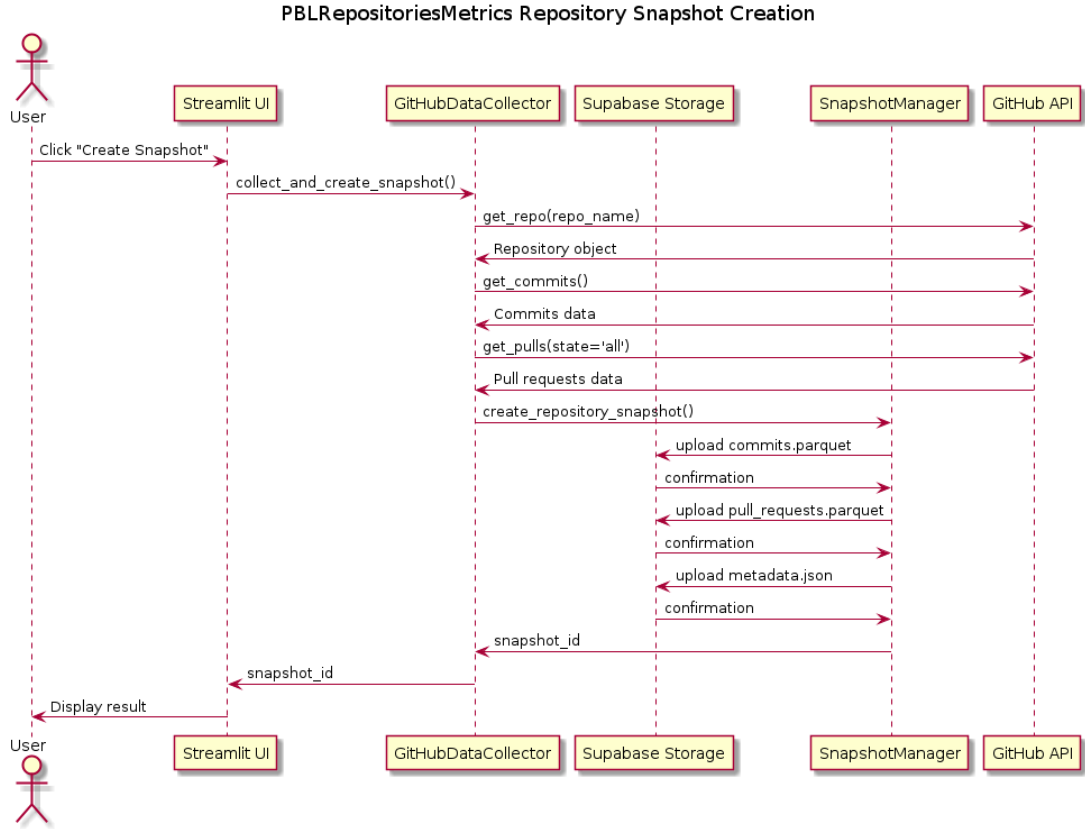
Figure 3: Sequence Diagram: PBLRepositoriesMetrics Repository Snapshot Creation Process
