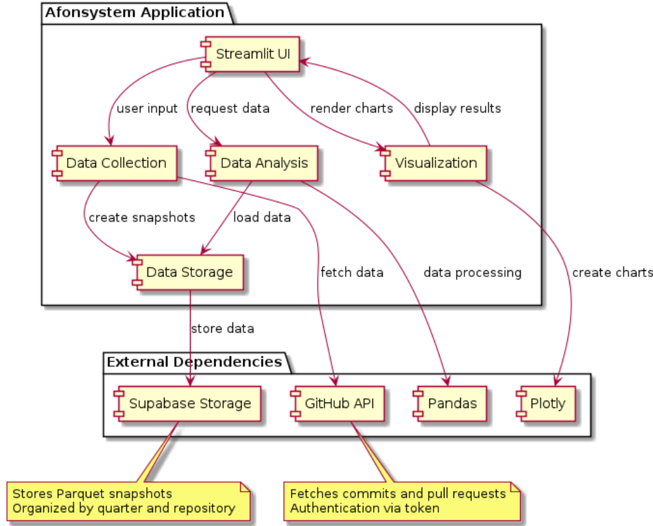
Figure 1: Component Diagram of PBLRepositoriesMetrics
