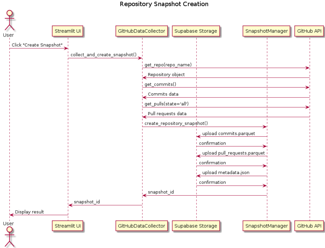
Figure 3: Sequence Diagram: Repository Snapshot Creation Process
