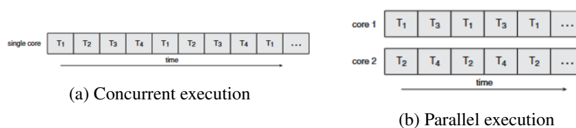
Figure 2.4: Conceptual distinction between concurrency and parallelism [29].
