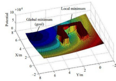
(c) Potential field exhibiting local minima induced by obstacles [38].
