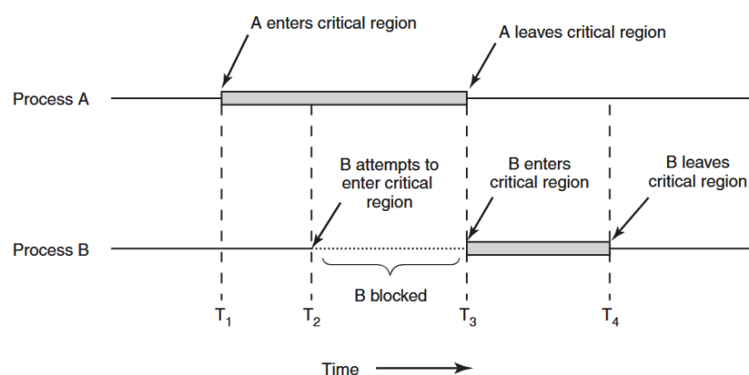
Figure 2.6: Illustration of mutual exclusion in a critical section. While Process A executes its critical section, Process B is blocked until the resource becomes available [30].
